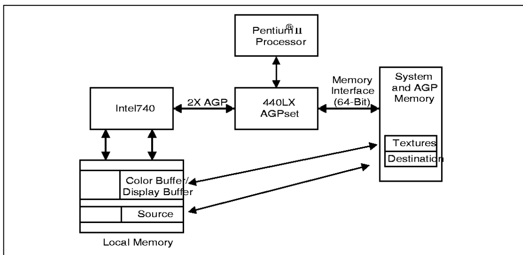
Figure 1-5. The Intel740™ Graphics Accelerator Functioning as Two Memory Controllers
