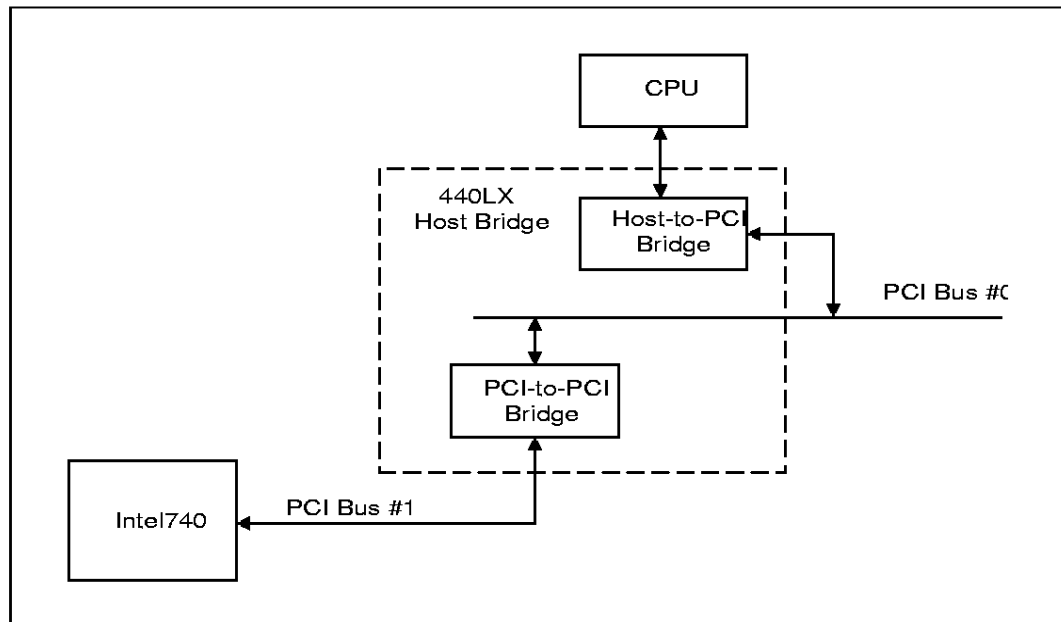
Figure 3-1. PCI Bus Hierarchy (Using 82443LX as Host Bridge)
