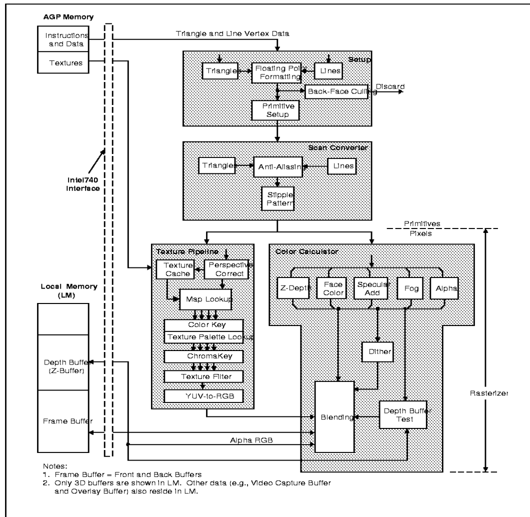
Figure 4-2. The Intel740Graphics Accelerator's 3D Pipeline (Parallel Data Paths)
