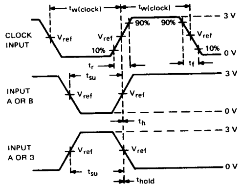
SWITCHING TIMES VOLTAGE WAVEFORMS
