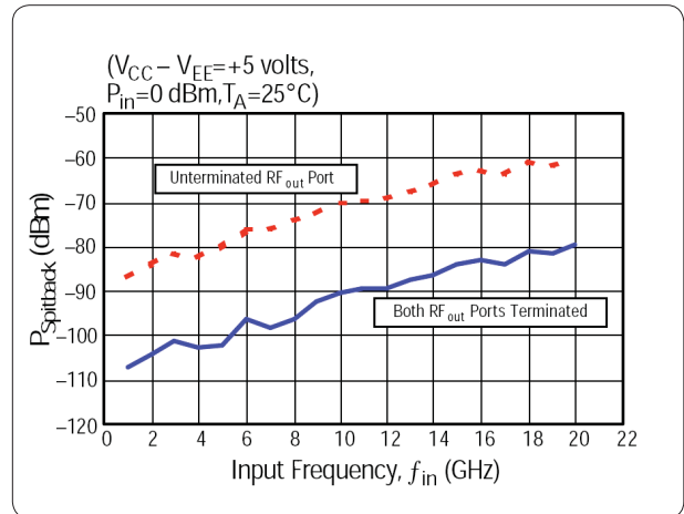
Figure 9. Typical "Spitback" power P(f_{\text{out}}) appearing at RF input port
