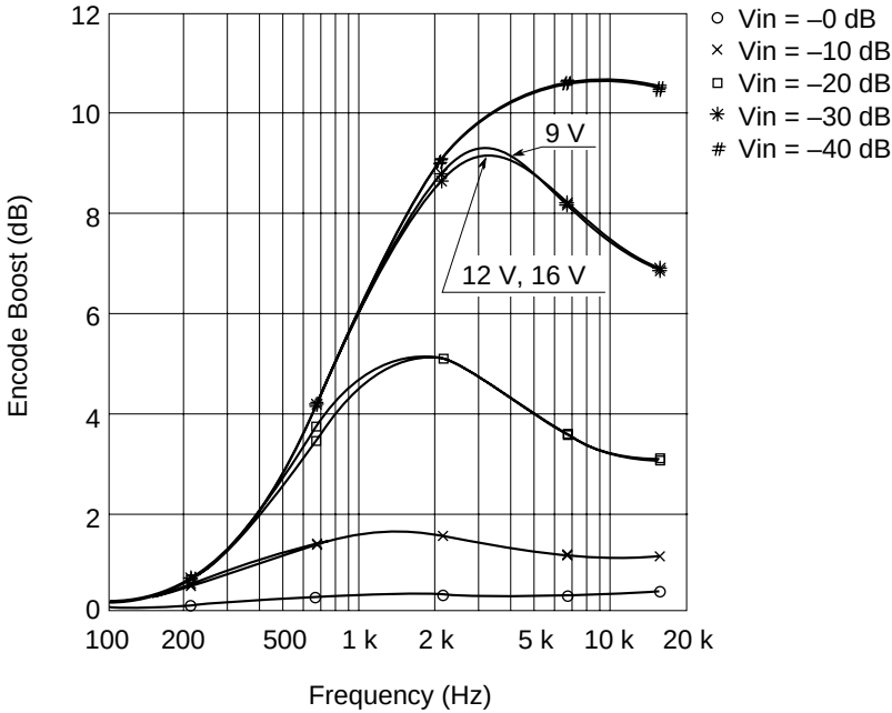
Encode Boost vs. Frequency (NR-B, V_{cc} = 9 V, 12 V, 16 V)
