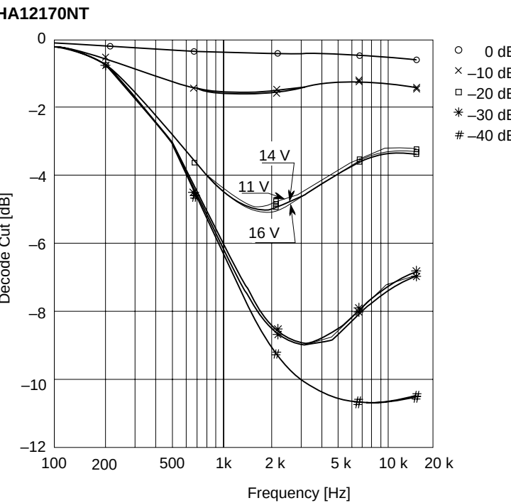
Decode Cut vs. Frequency (NR-B V_{CC} = 11 V, 14 V, 16 V)
