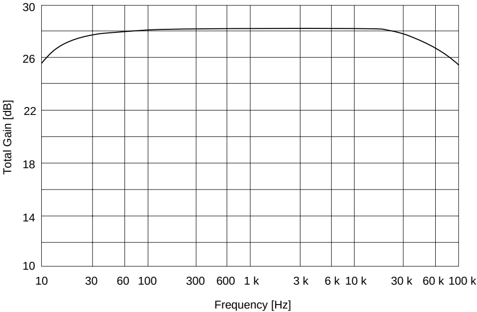
Total Gain vs. Frequency (PB MODE PBOUT NR-OFF V_{CC} = 14\text{ V} )
