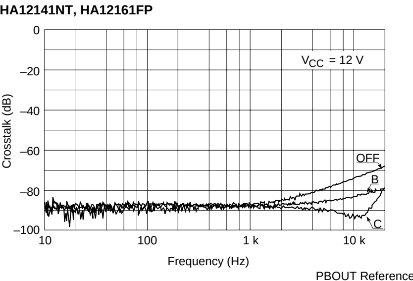
Crosstalk vs. Frequency (PB MODE R→L)
