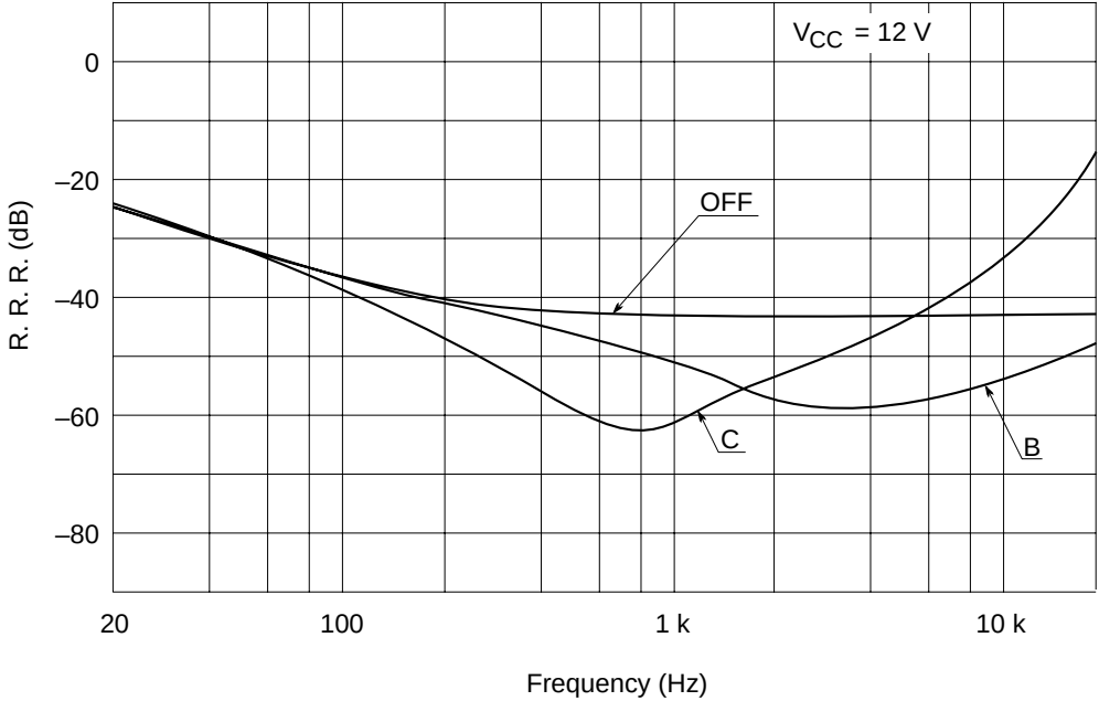
Ripple Rejection Ratio vs. Frequency (PB MODE PBOUT)
