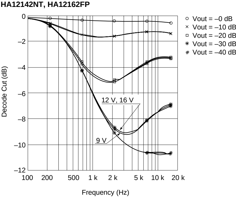
Decode Cut vs. Frequency (NR-B, V_{cc} = 9V, 12 V, 16 V)
