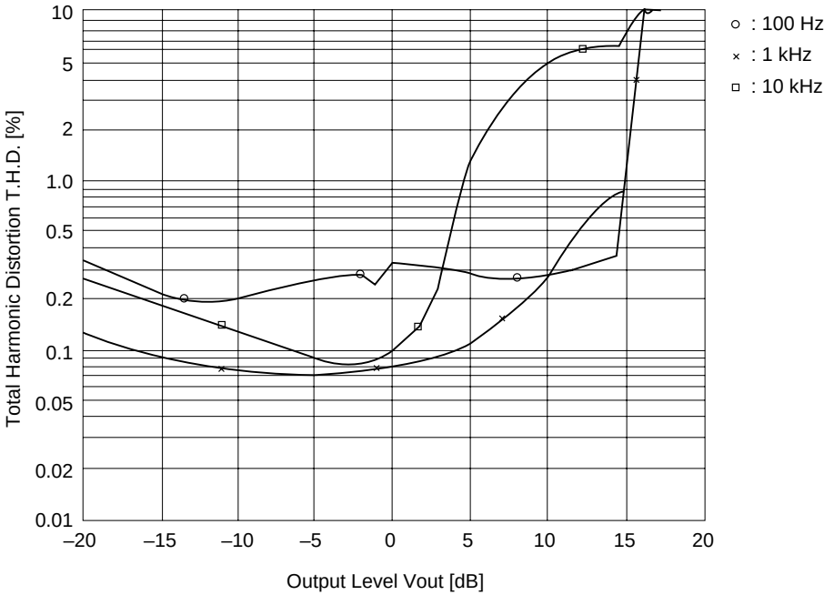
Total Harmonic Distortion vs. Output Level (PB MODE NR-C V_{cc} = 14\text{ V} )
