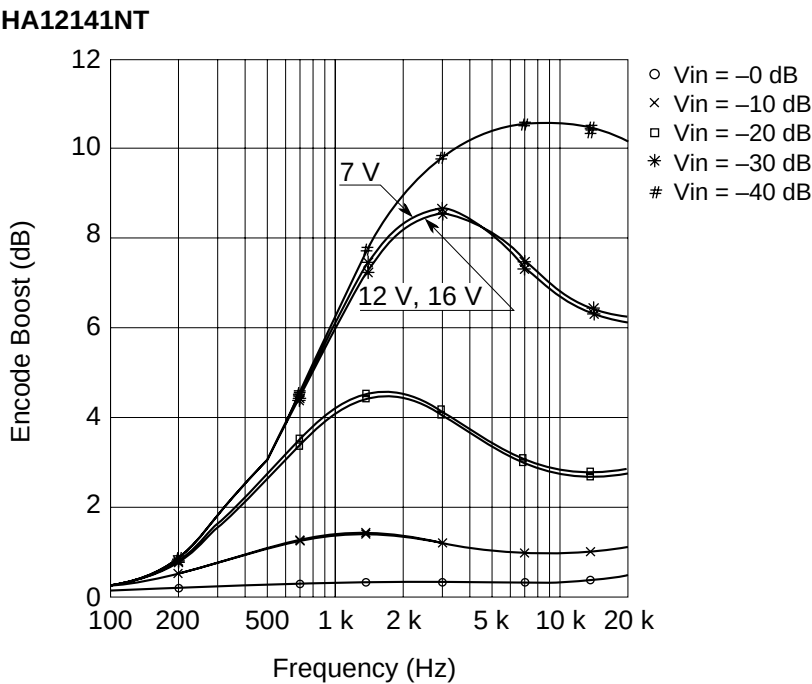
Encode Boost vs. Frequency (NR-B V CC = 7V, 12 V, 16 V)
