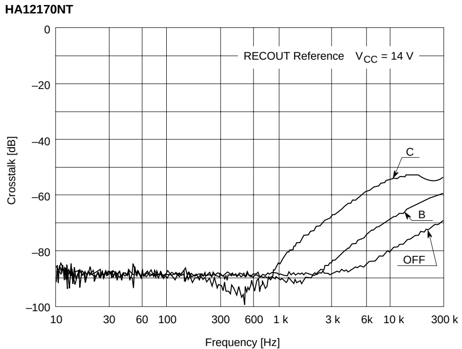
Crosstalk vs. Frequency (REC MODE R↔L)
