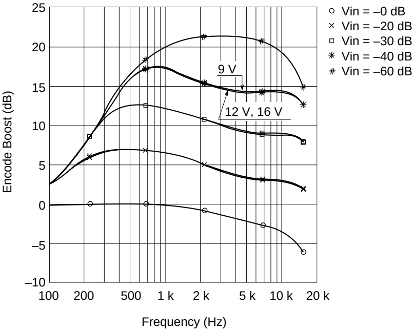
Encode Boost vs. Frequency (NR-C, V_{cc} = 9 V, 12 V, 16 V)
