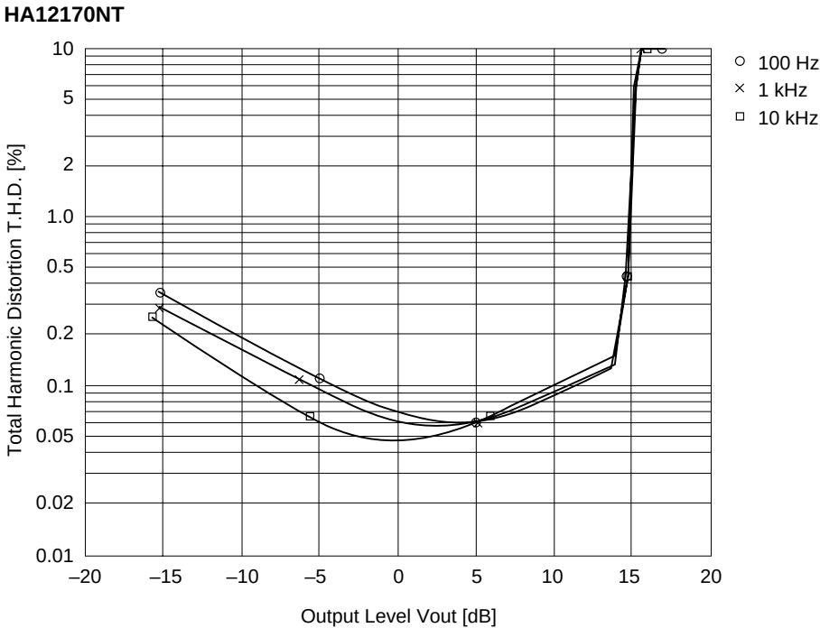
Total Harmonic Distortion vs. Output Level (REC MODE NR-B V_{CC} = 14\text{ V} )
