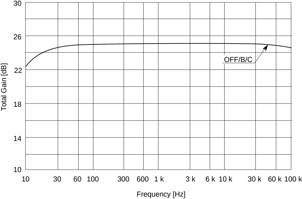
Total Gain vs. Frequency (REC MODE PBOUT V_{cc} = 14\text{ V} )
