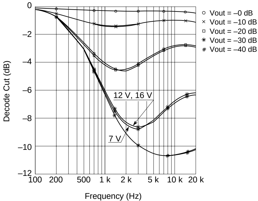
Decode Cut vs. Frequency (NR-B V_{cc} = 7 V, 12 V, 16 V)
