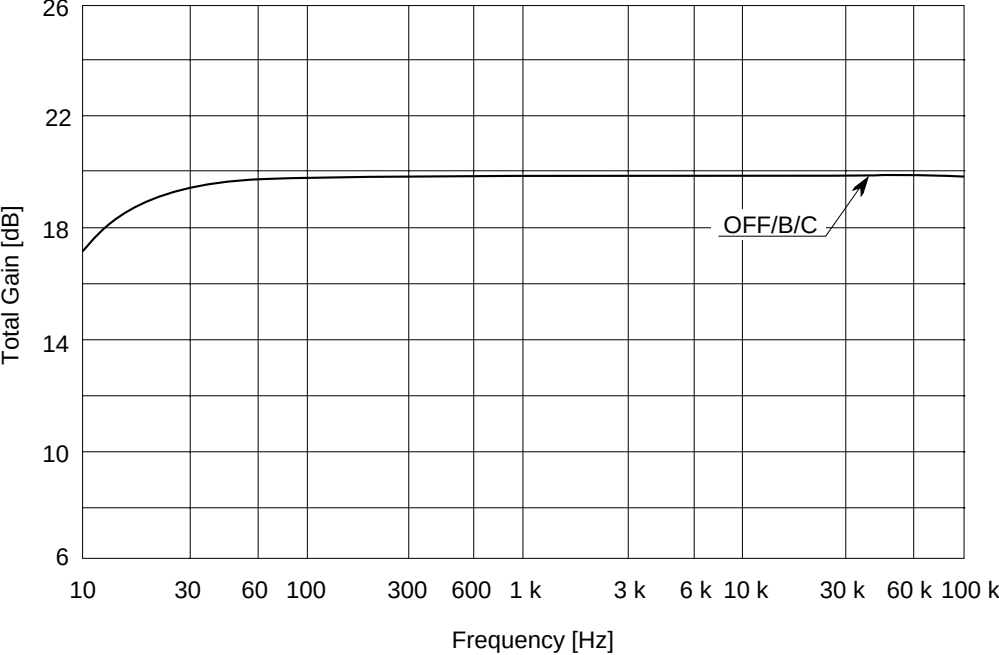
Total Gain vs. Frequency (PB MODE RECOUNT V_{cc} = 14\text{ V} )
