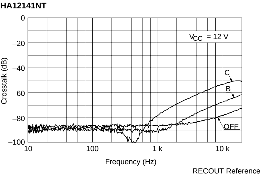
Crosstalk vs. Frequency (REC MODE R→L)
