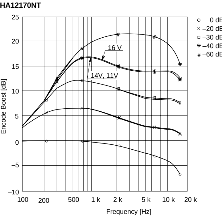
Encode Boost vs. Frequency (NR-C V_{CC} = 11 V, 14 V, 16 V)
