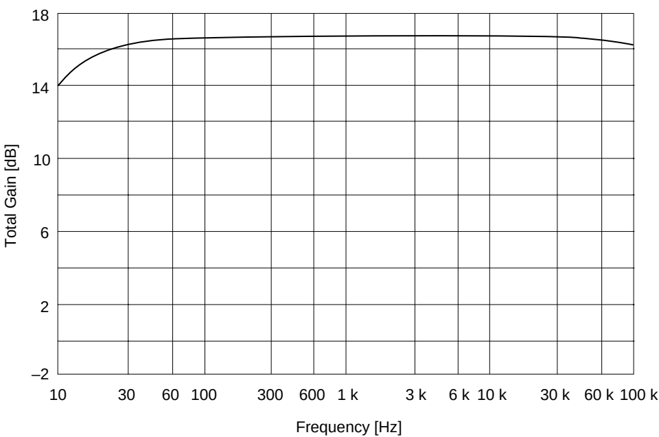
Total Gain vs. Frequency (REC MODE RECOUT NR-OFF V_{cc} = 14 V)
