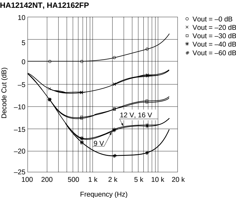
Decode Cut vs. Frequency (NR-C, V_{cc} = 9V, 12 V, 16 V)
