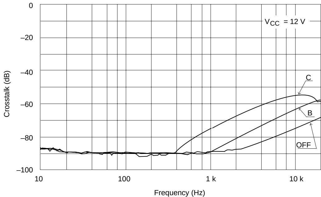
Crosstalk vs. Frequency (PB→REC)
