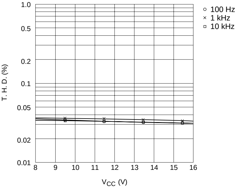
Total Harmonic Distortion vs. Supply Voltage (REC MODE NR-B)
