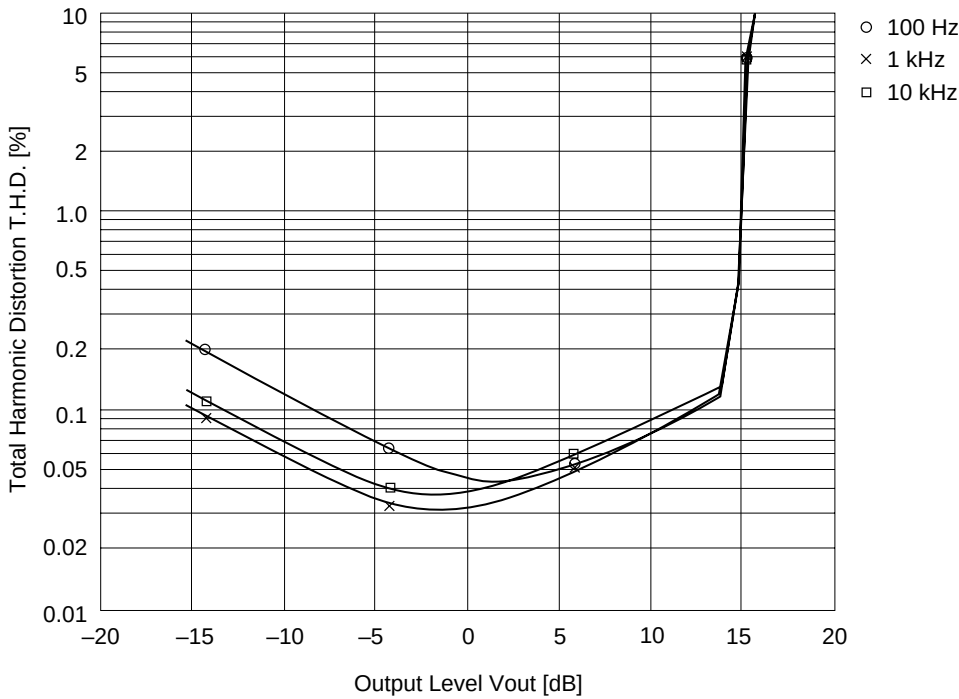
Total Harmonic Distortion vs. Output Level (REC MODE NR-OFF V_{CC} = 14\text{ V} )
