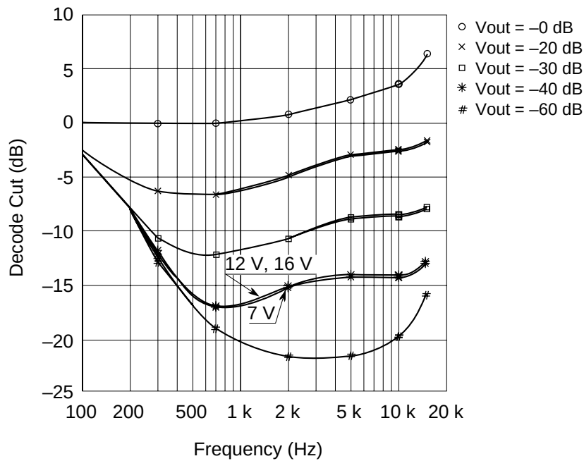
Decode Cut vs Frequency (NR-C V_{CC} = 7 V, 12 V, 16 V)
