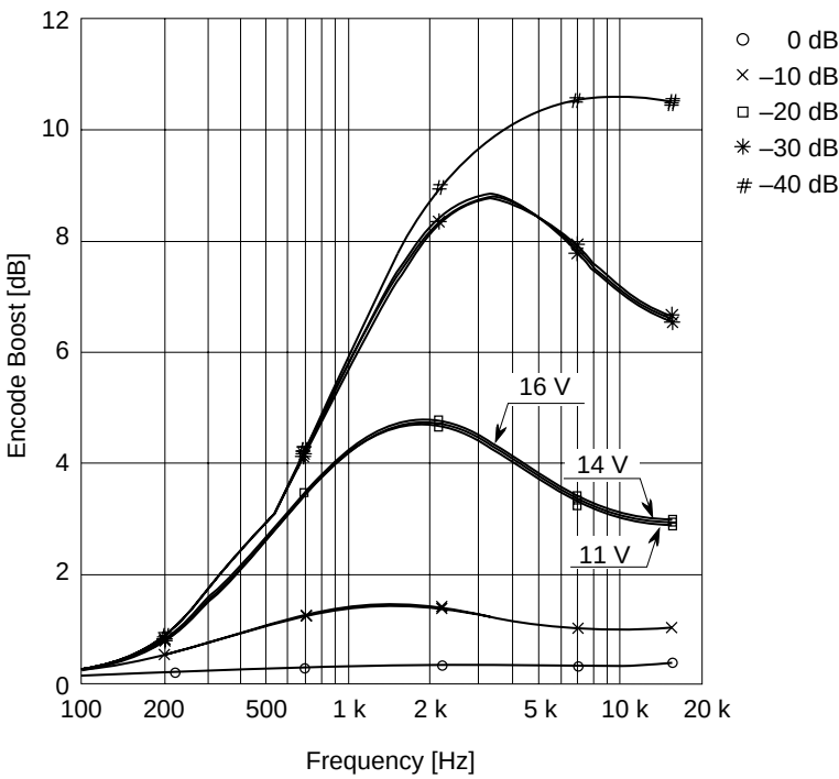
Encode Boost vs. Frequency (NR-B V_{CC} = 11V, 14V, 16V )
