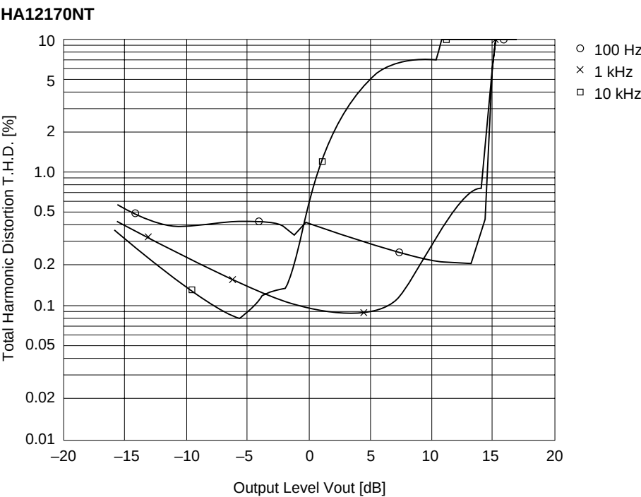
Total Harmonic Distortion vs. Output Level (REC MODE NR-C V_{CC} = 14\text{ V} )
