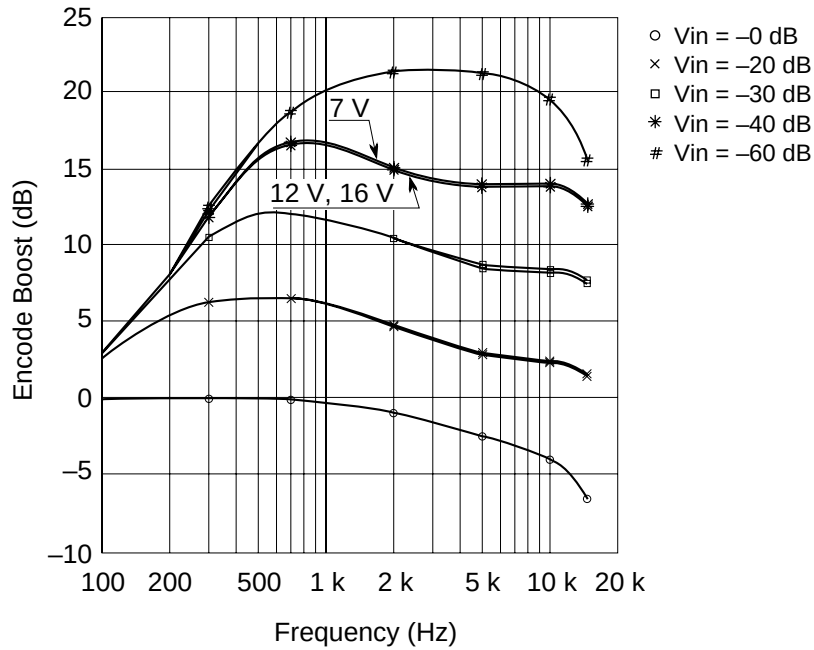
Encode Boost vs. Frequency (NR-C V_{cc} = 7 V, 12 V, 16 V)
