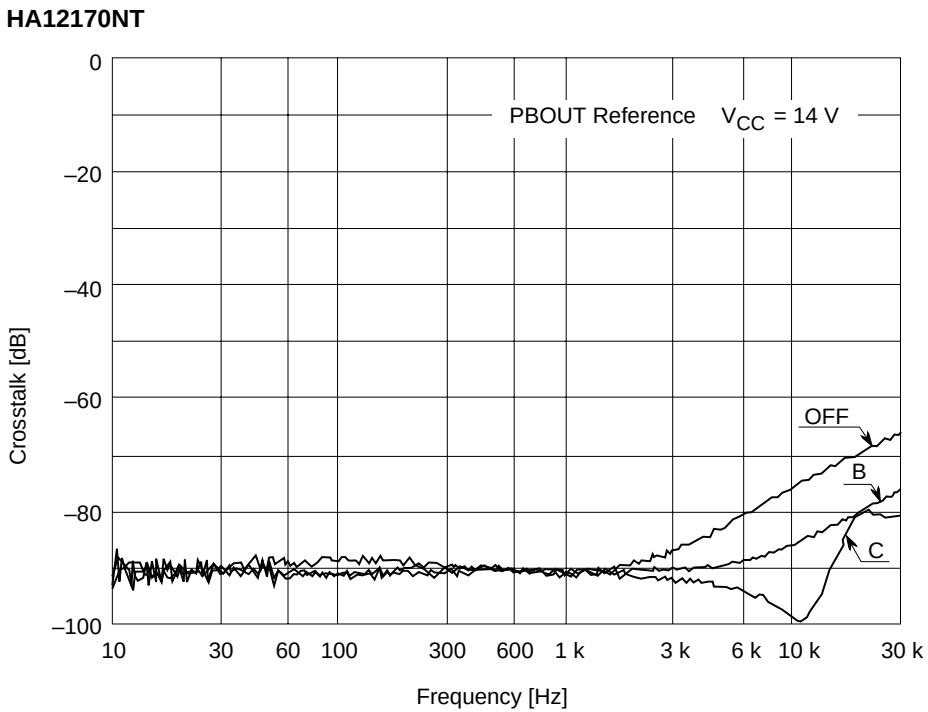
Crosstalk vs. Frequency (PB MODE R↔L)
