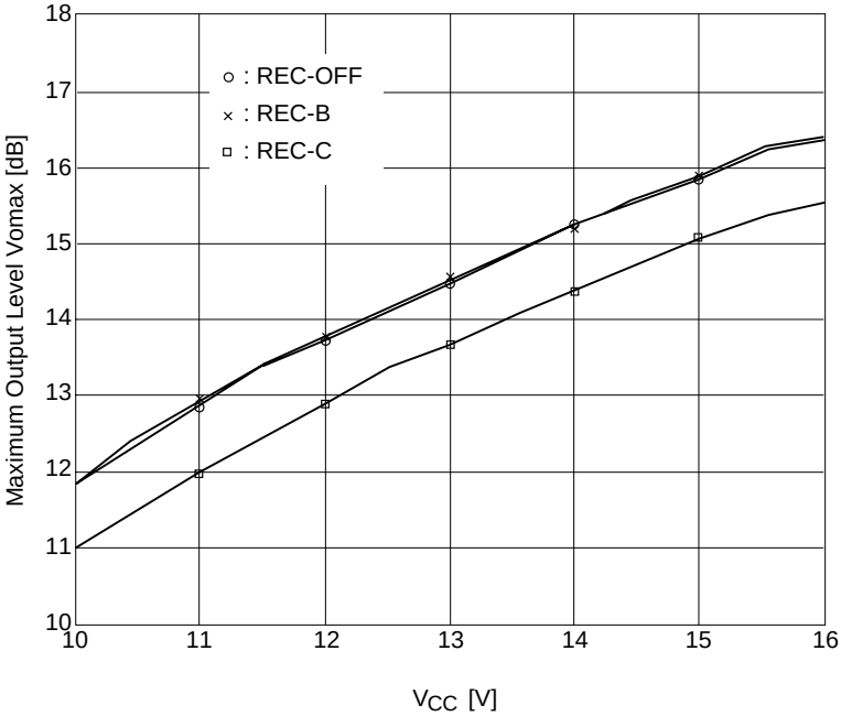
Maximum Output Level vs. Supply Voltage (REC MODE)
