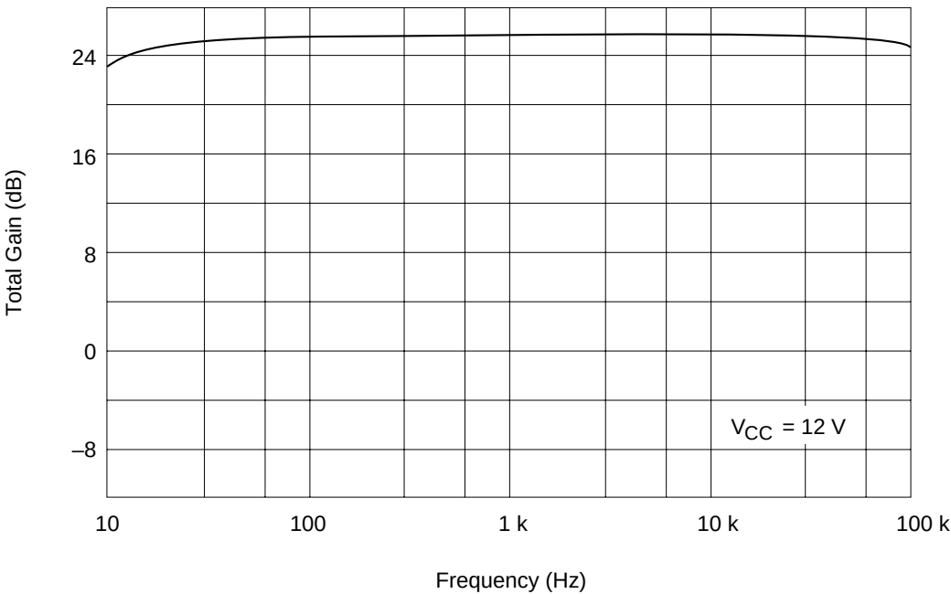
Total Gain vs. Frequency (PB MODE PBOUT NR-OFF)
