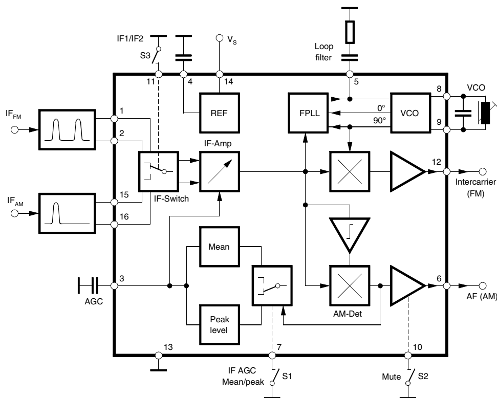
Figure 1. Block Diagram
