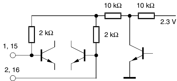
Figure 4. Sound IF Inputs (Pins 1 and 2 Respectively 15, 16)
