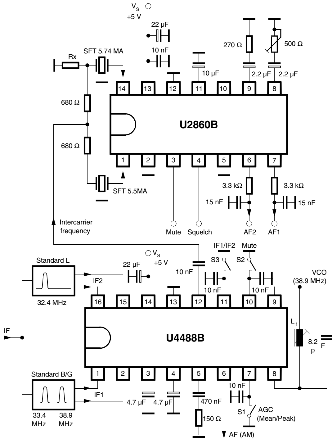
Figure 3. Test Circuit
