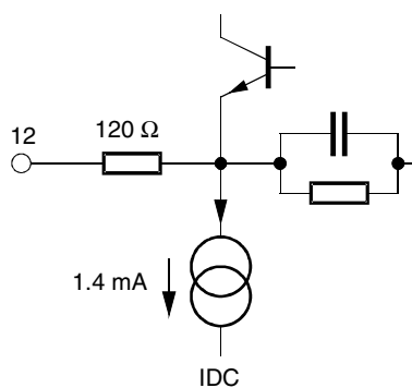
Figure 13. Intercarrier Output (Pin 12)
