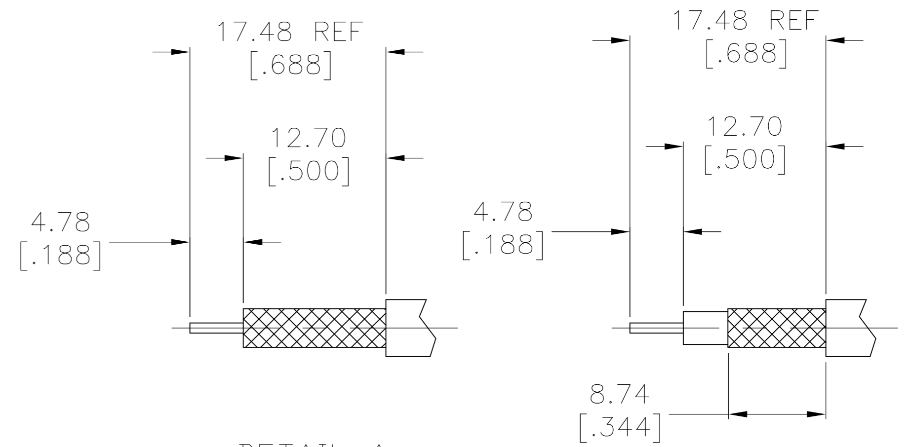
DETAIL A
