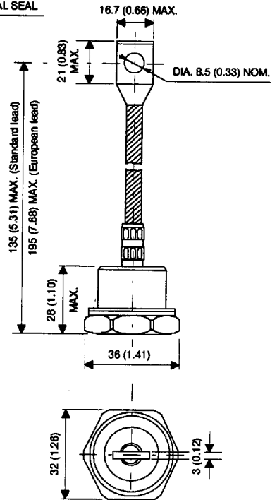
70/300UF DO-205AB (DO-9) Flat Base
