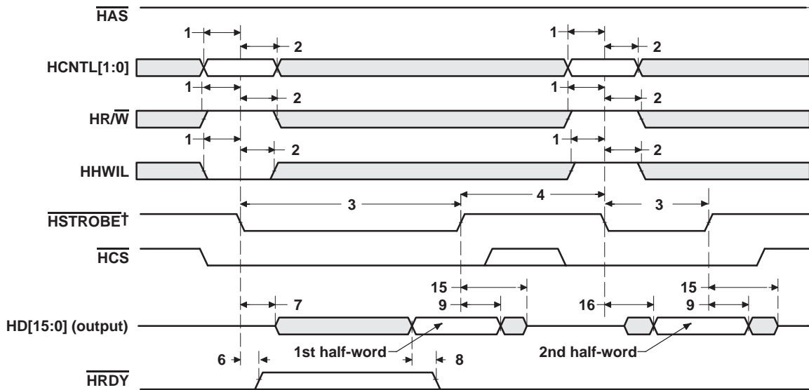
Figure 34. HPI16 Read Timing ( \overline{\text{HAS}} Not Used, Tied High)
