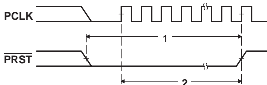
Figure 43. PCI Reset ( \overline{\text{PRST}} ) Timing
