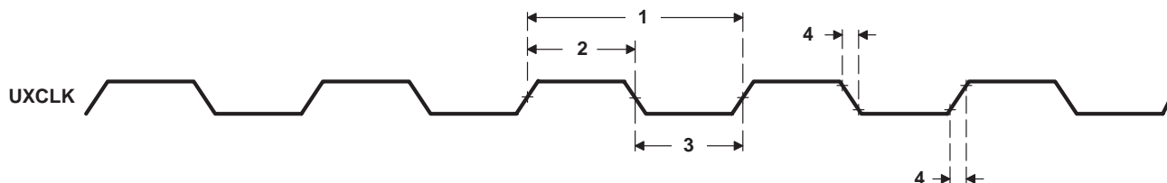
Figure 52. UXCLK Timing
