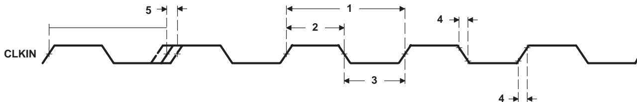
Figure 11. CLKIN Timing
