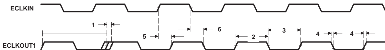
Figure 15. ECLKOUT1 Timing for EMIFA and EMIFB Modules
