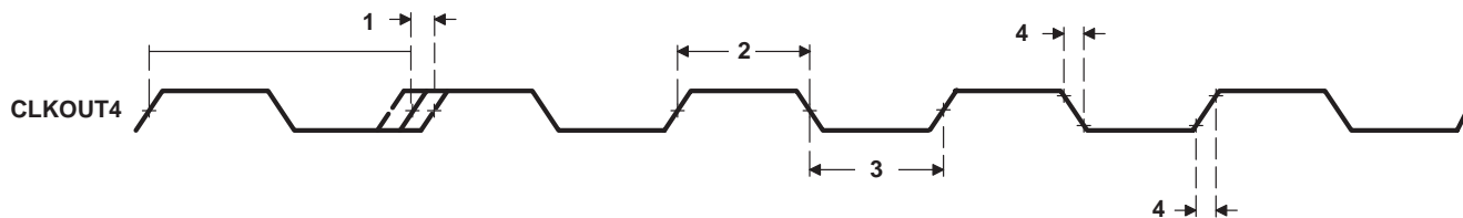
Figure 12. CLKOUT4 Timing
