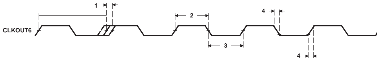
Figure 13. CLKOUT6 Timing
