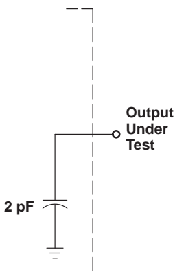
Figure 7. AC Timing Reference Circuit for ac Timing Measurements
