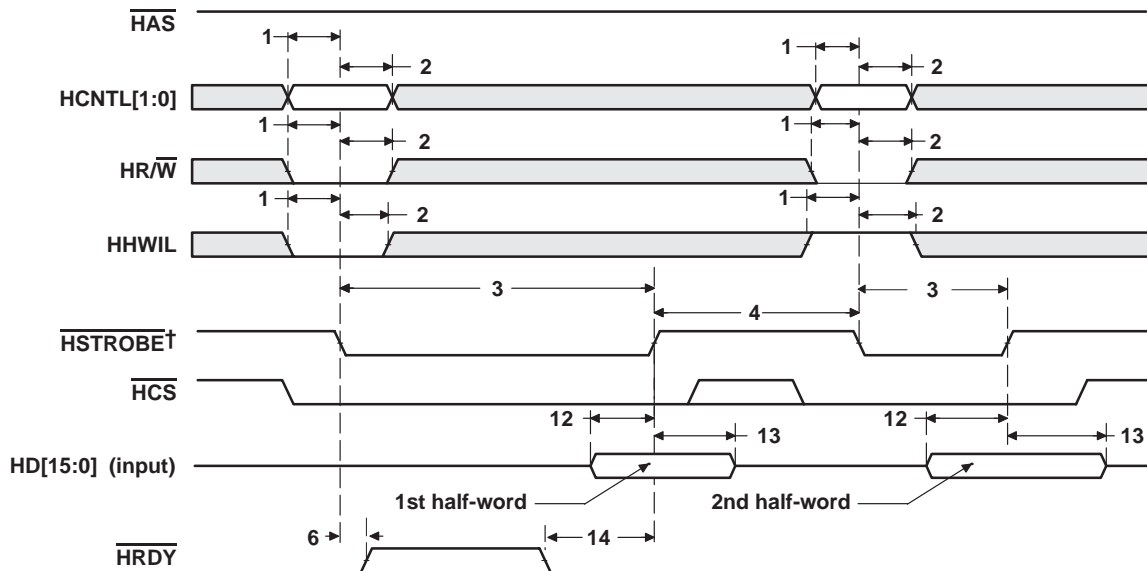
Figure 36. HPI16 Write Timing ( \overline{\text{HAS}} Not Used, Tied High)
