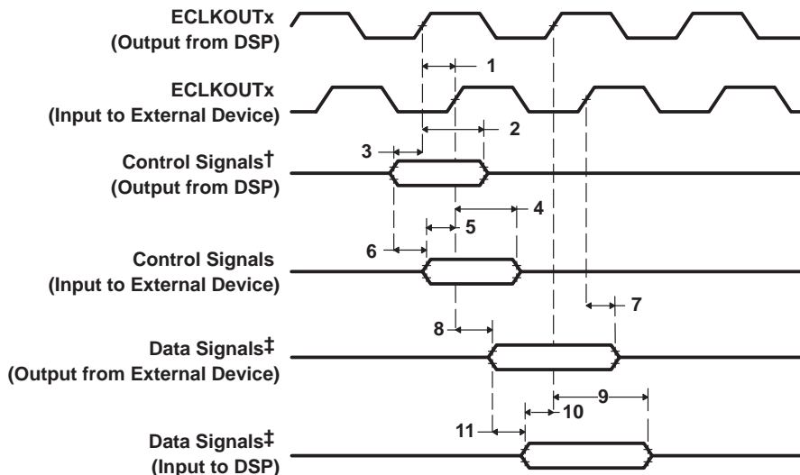
Figure 10. Board-Level Input/Output Timings
