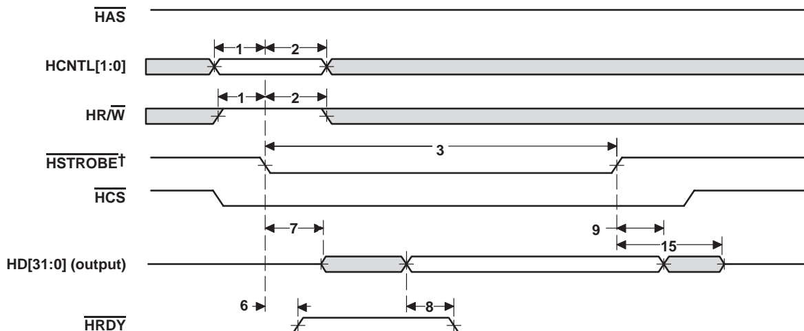
Figure 38. HPI32 Read Timing ( \overline{\text{HAS}} Not Used, Tied High)
