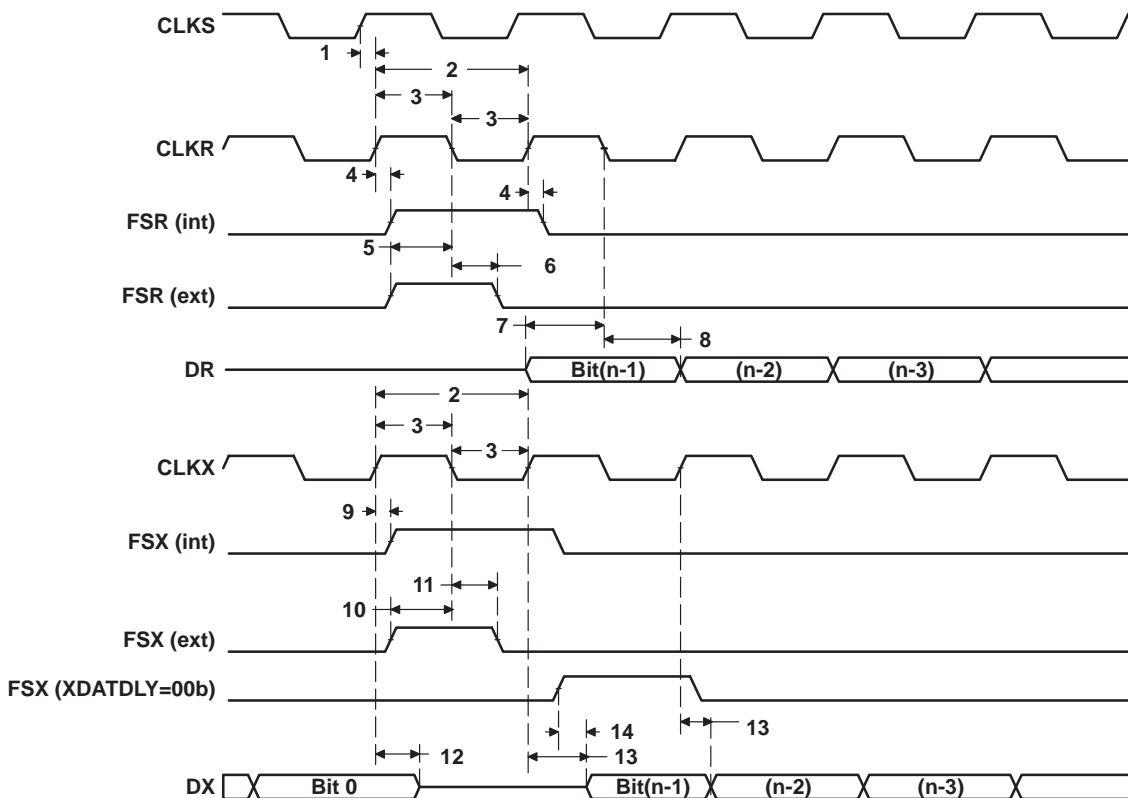
Figure 46. McBSP Timing
