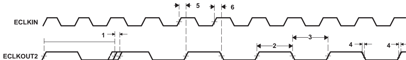
Figure 16. ECLKOUT2 Timing for the EMIFA and EMIFB Modules
