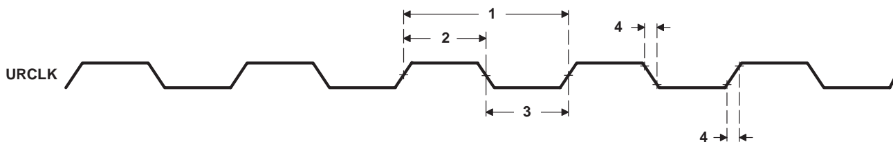
Figure 53. URCLK Timing
