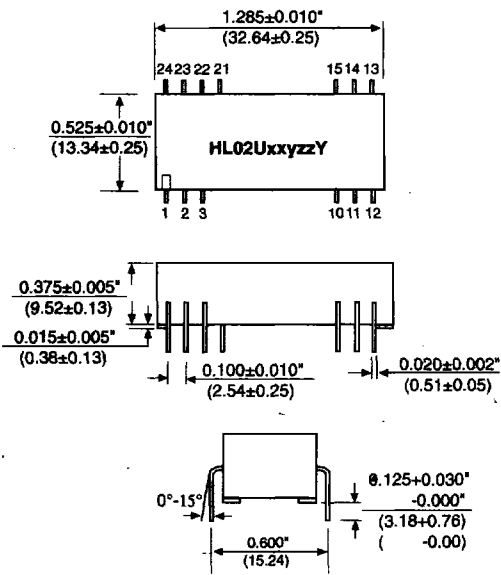
DIP PACKAGE
