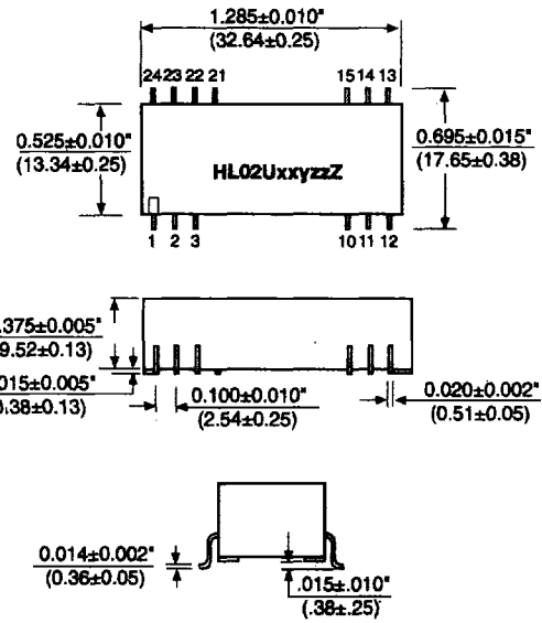
SMD PACKAGE
