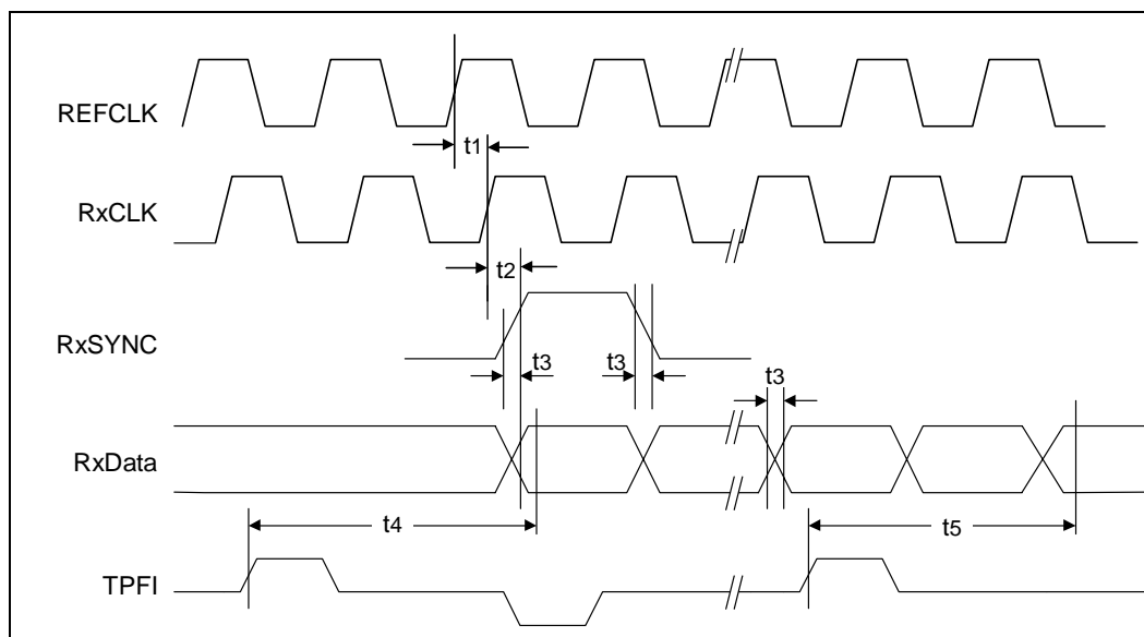
Figure 46. SS-SMII - 100BASE-TX Receive Timing
