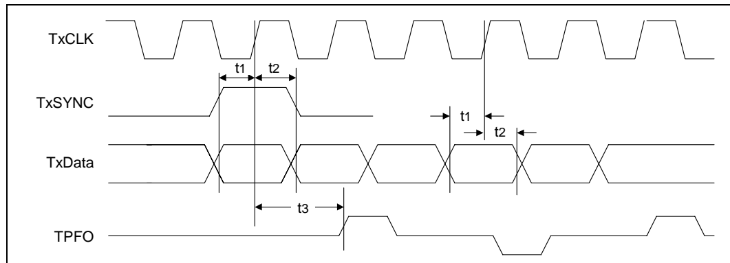
Figure 47. SS-SMII - 100BASE-TX Transmit Timing
