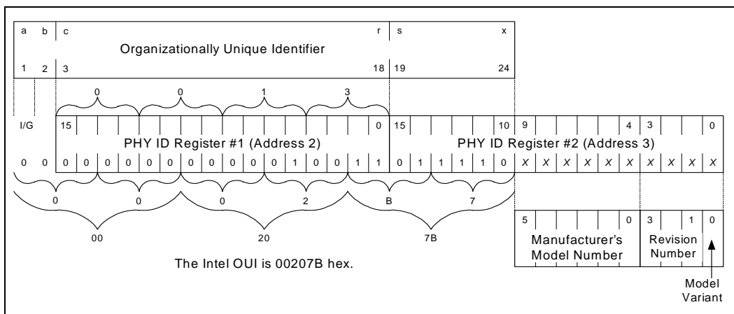
Figure 64. PHY Identifier Bit Mapping
