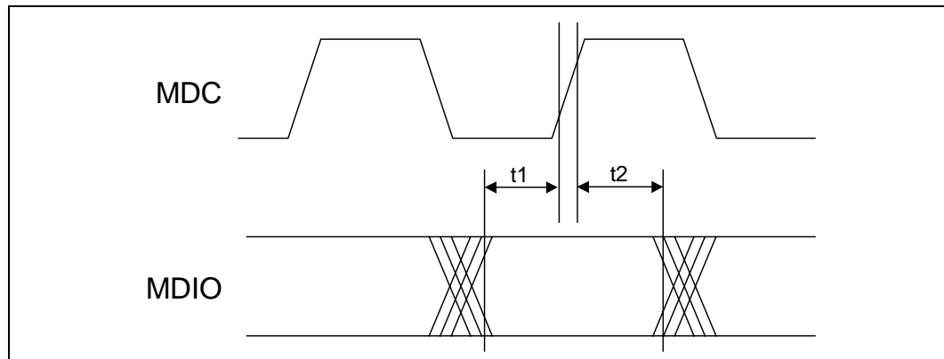
Figure 61. MDIO Read Timing (MDIO Sourced by PHY)
