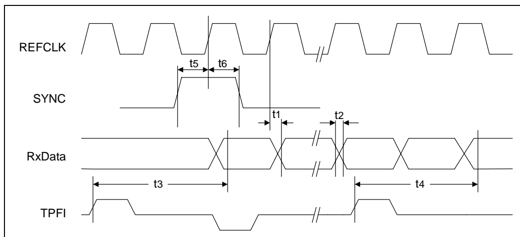
Figure 40. SMII - 100BASE-TX Receive Timing
