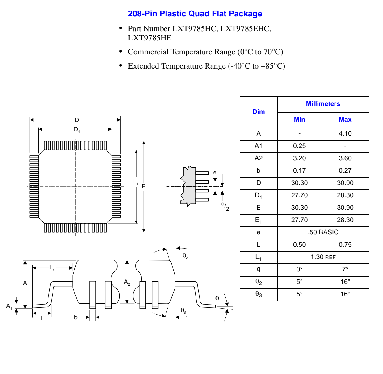
Figure 65. LXT9785/9785E 208-Pin PQFP Plastic Package Specification
