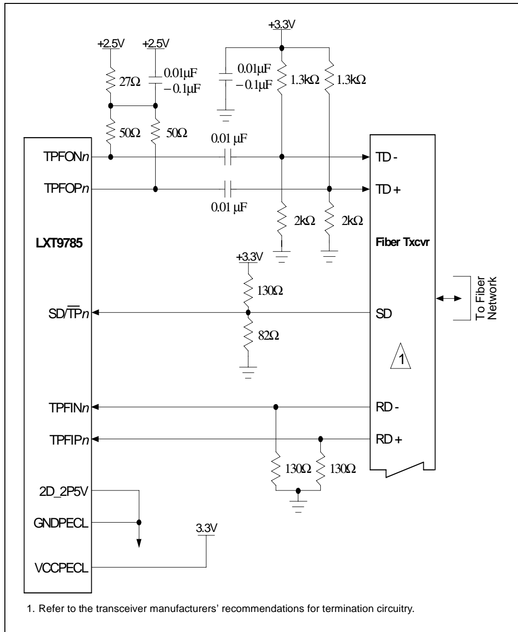
Figure 37. Typical LXT9785/9785E to 3.3V Fiber Transceiver Interface Circuitry
