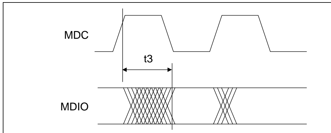
Figure 61. MDIO Read Timing (MDIO Sourced by PHY)
