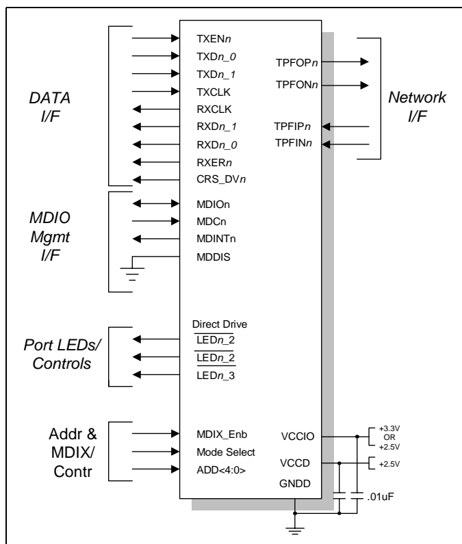
Figure 8. LXT9785/9785E Interfaces
