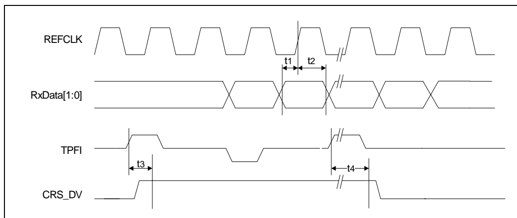
Figure 54. RMII - 100BASE-FX Receive Timing
