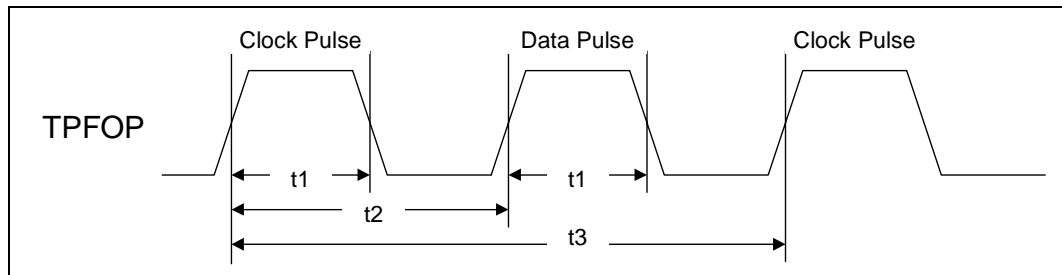
Figure 59. Fast Link Pulse Timing
