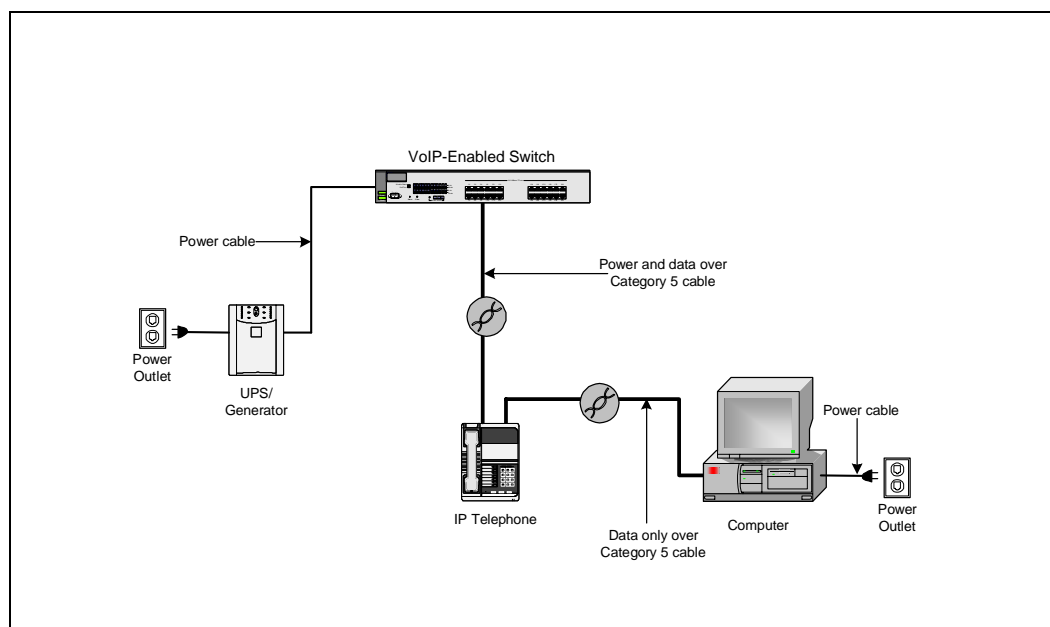
Figure 30. Typical IP Telephone System Connection
