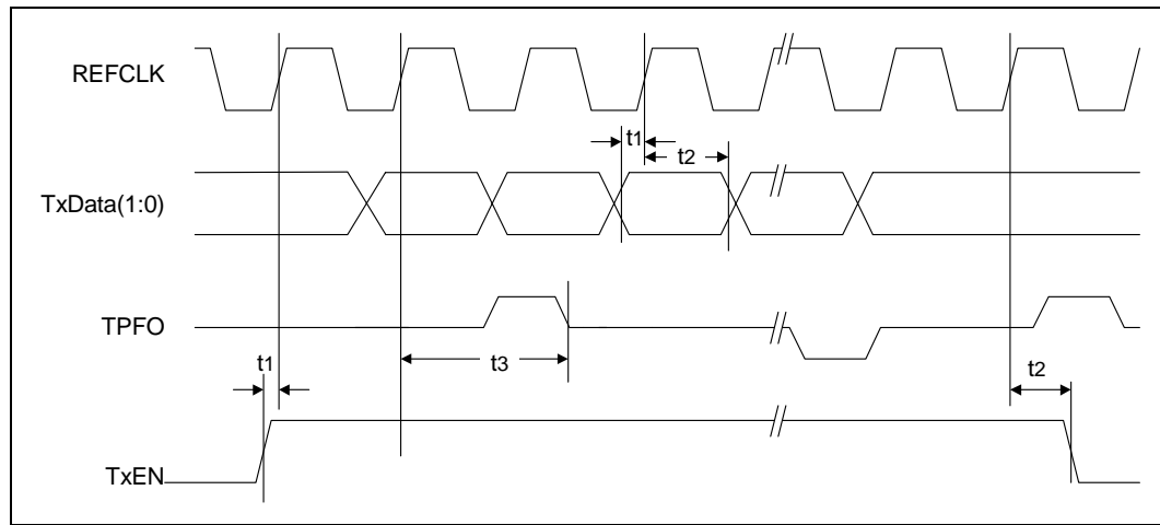
Figure 57. RMII - 10BASE-T Transmit Timing
