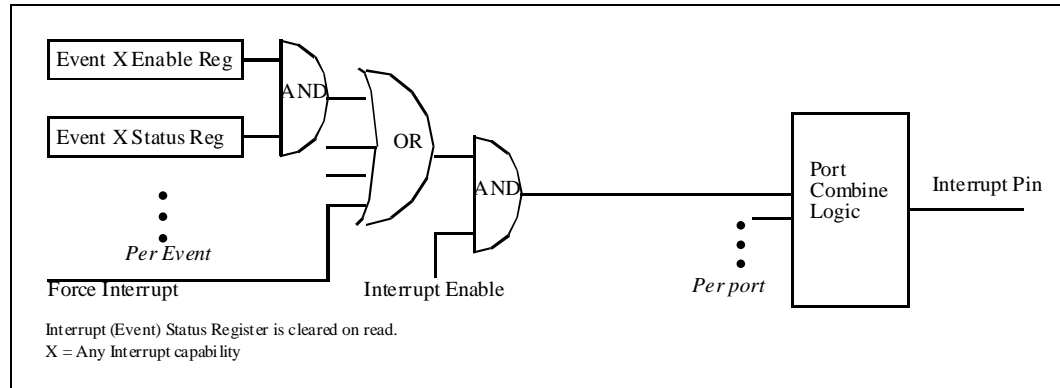
Figure 13. Interrupt Logic
