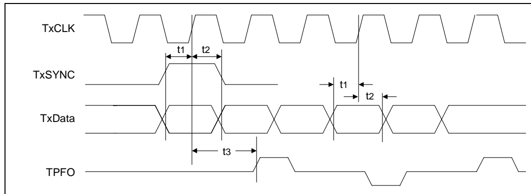
Figure 49. SS-SMII - 100BASE-FX Transmit Timing
