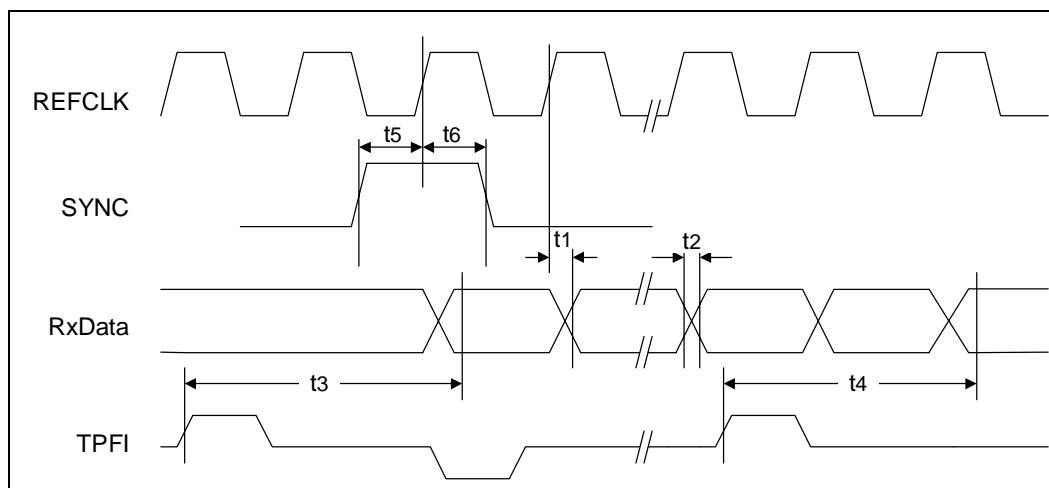
Figure 44. SMII - 10BASE-T Receive Timing
