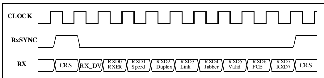
Figure 20. Serial MII Receive Synchronization
