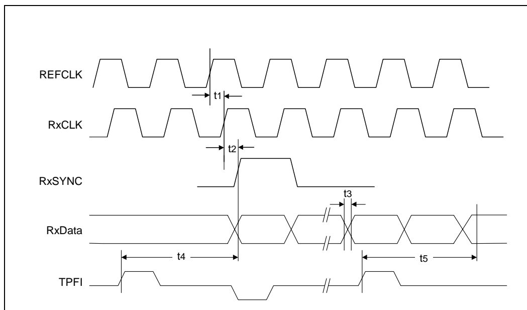
Figure 50. SS-SMII - 10BASE-T Receive Timing
