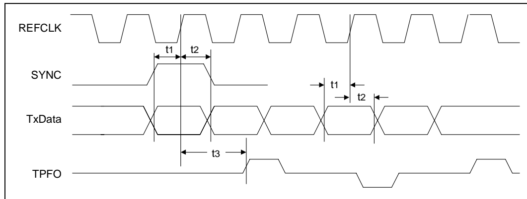
Figure 41. SMII - 100BASE-TX Transmit Timing
