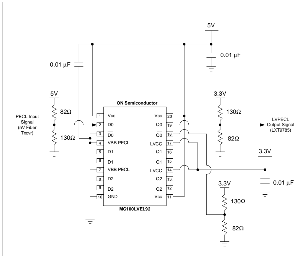
Figure 39. ON Semiconductor Triple PECL-to-LVPECL Translator
