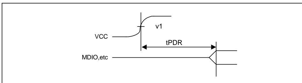
Figure 62. Power-Up Timing
