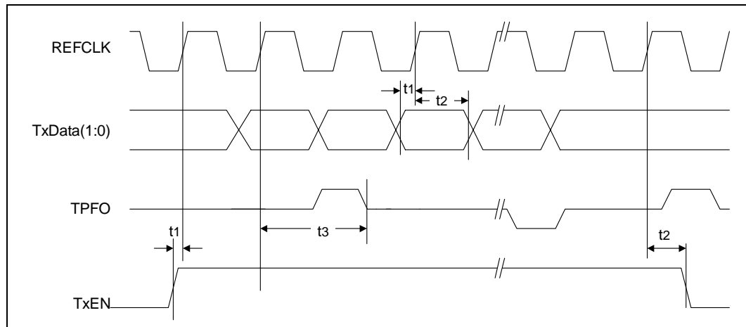
Figure 55. RMII - 100BASE-FX Transmit Timing
