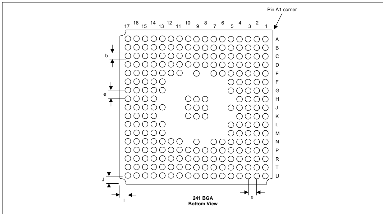
Figure 67. LXT9785/9785E 241-Ball PBGA Package Specs - Bottom View (LXT9785BC)
