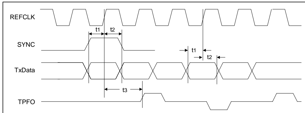
Figure 43. SMII - 100BASE-FX Transmit Timing
