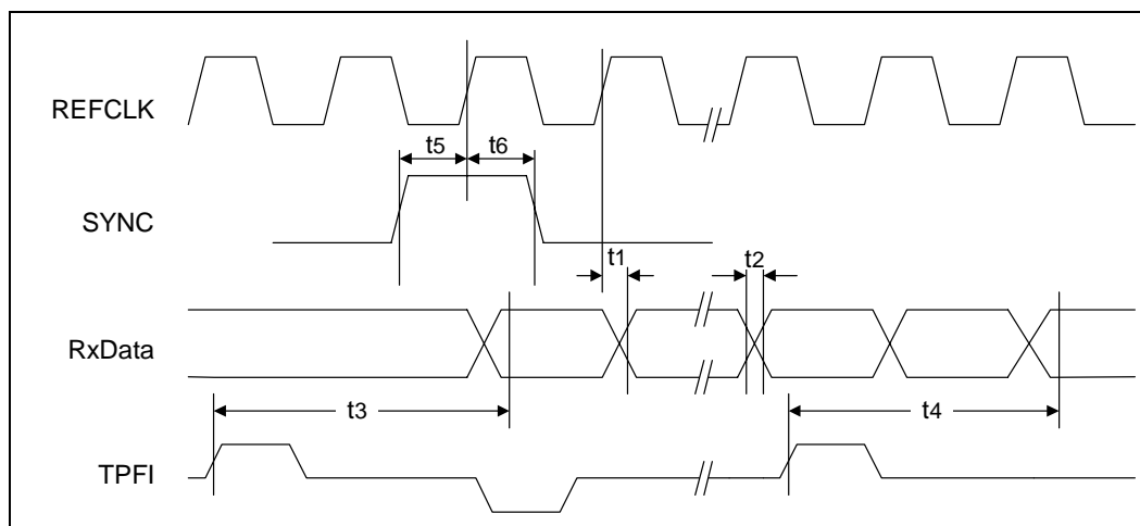
Figure 42. SMII - 100BASE-FX Receive Timing
