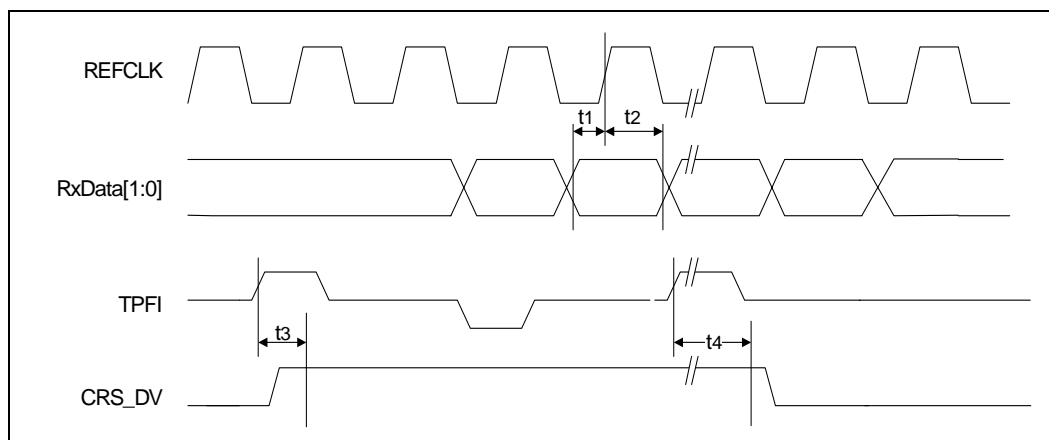
Figure 56. RMII - 10BASE-T Receive Timing
