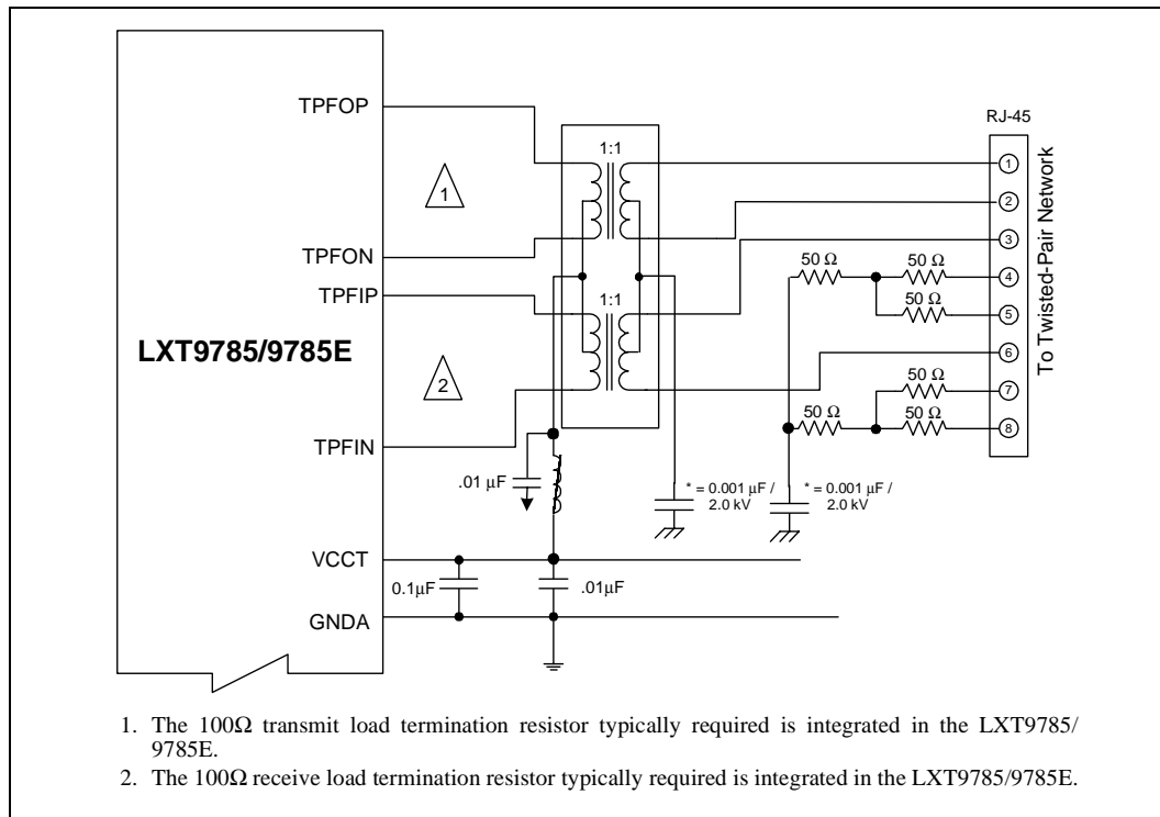
Figure 36. Typical Twisted-Pair Interface
