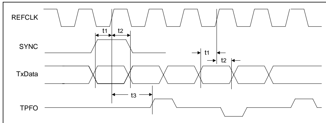
Figure 45. SMII - 10BASE-T Transmit Timing
