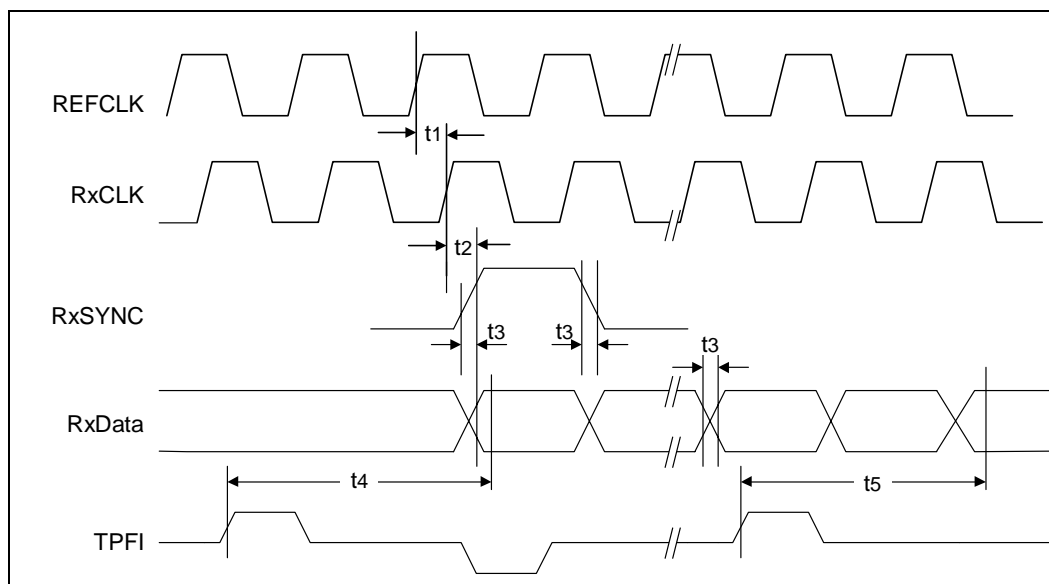
Figure 48. SS-SMII - 100BASE-FX Receive Timing
