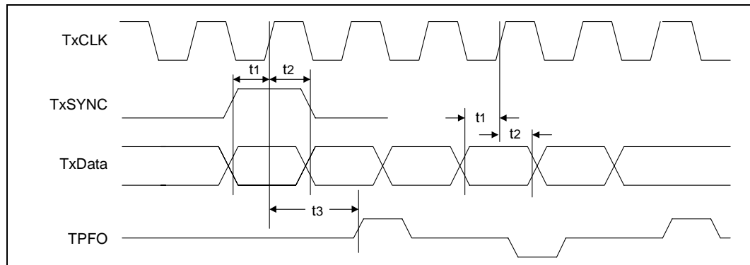
Figure 51. SS-SMII - 10BASE-T Transmit Timing
