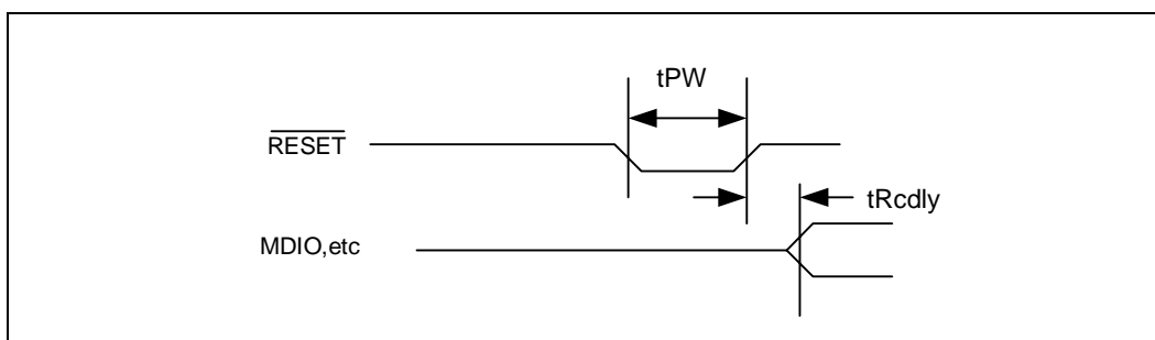
Figure 63. Reset Recovery Timing
