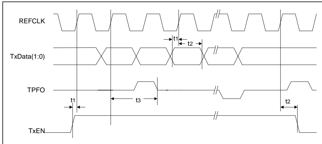
Figure 53. RMII - 100BASE-TX Transmit Timing
