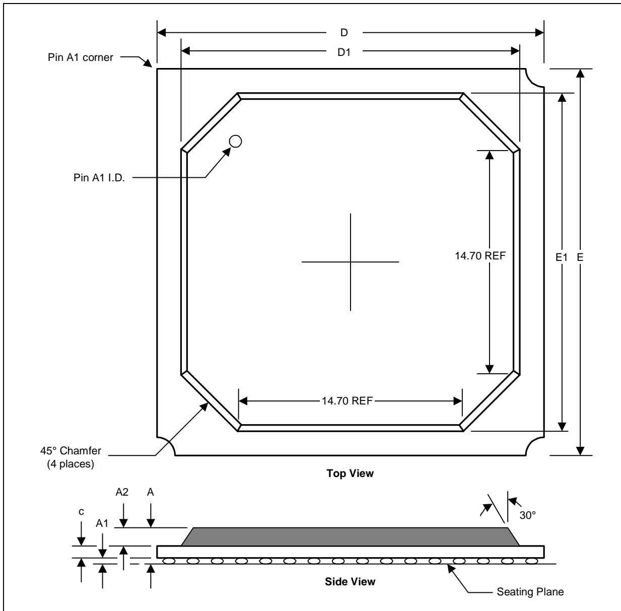
Figure 66. LXT9785/9785E 241-Ball PBGA Package Specs - Top/Side View(LXT9785BC)
