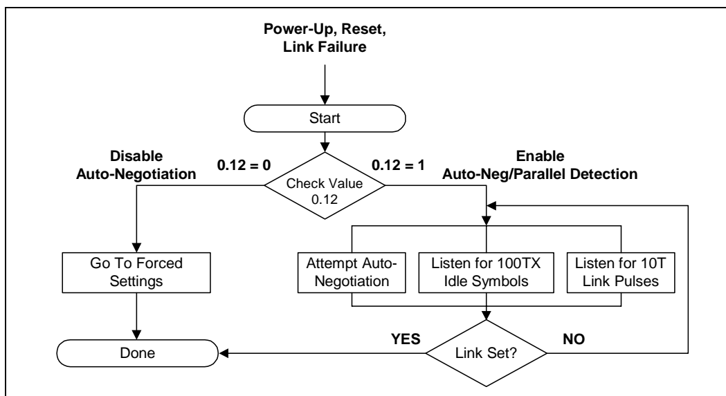
Figure 15. Auto-Negotiation Operation
