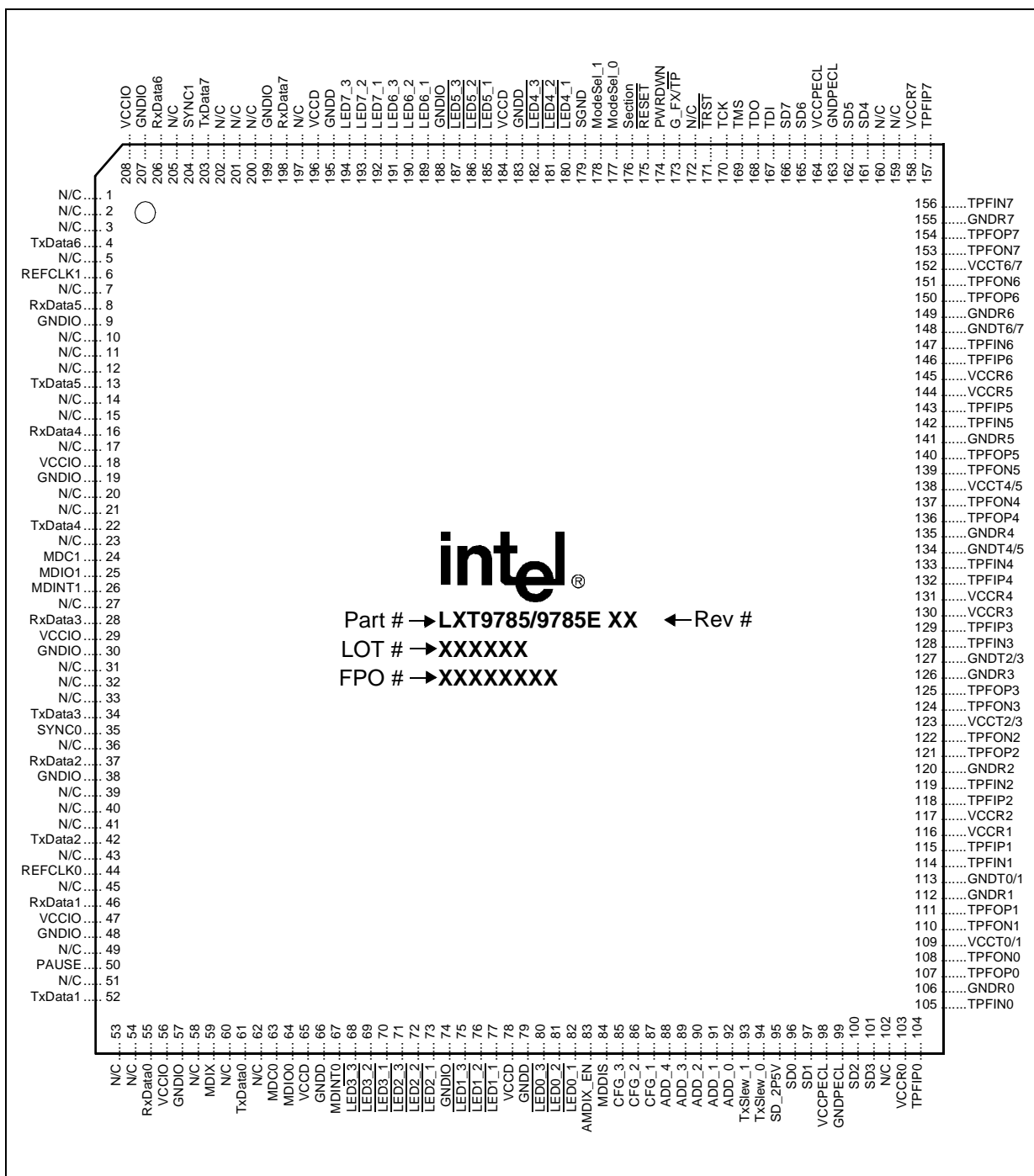
Figure 3. LXT9785/9785E SMII 208-Pin QQFP Assignments
