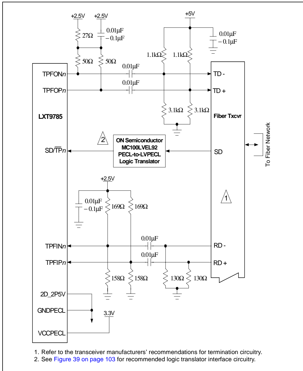
Figure 38. Typical LXT9785/9785E to 5V Fiber Transceiver Interface Circuitry
