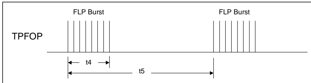
Figure 59. Fast Link Pulse Timing
