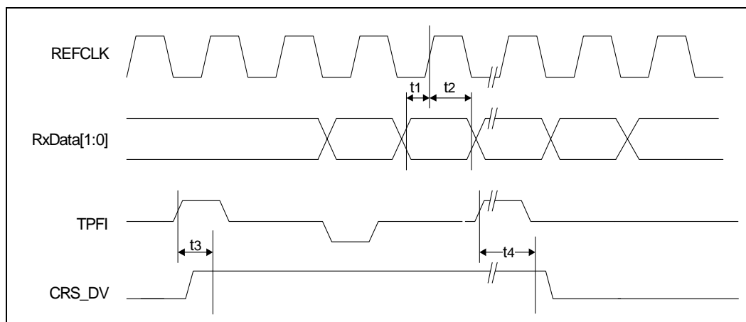
Figure 52. RMII - 100BASE-TX Receive Timing
