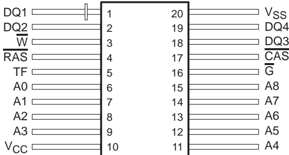
HK PACKAGE (TOP VIEW)
