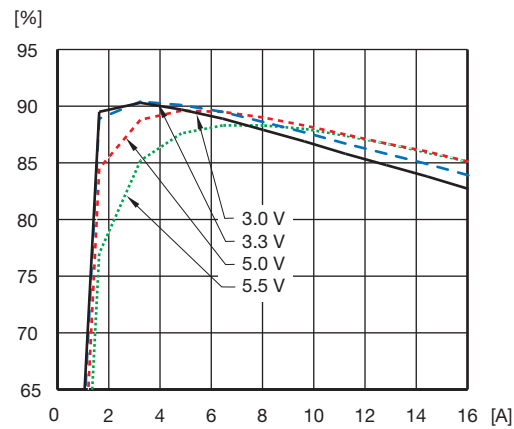
Efficiency vs. load current and input voltage at T_{re} = +25\text{ }^{\circ}\text{C}
