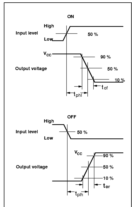
Figure 3. Timing diagram, input vs. output. V_{CC} = 24V .
