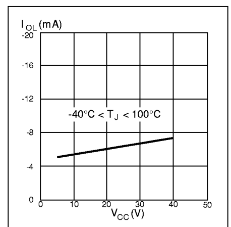
Figure 12. Output leakage current vs. supply voltage. 0 V \leq V_{IN} \leq 0.8 V . Output = 0 V.
