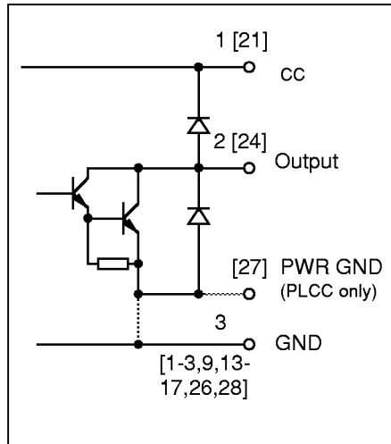
Figure 16. Output stage.
