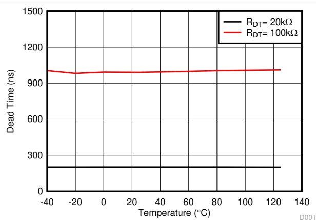
Figure 6-27. Dead Time vs. Temperature (with R_{DT} = 20\text{ k}\Omega and 100\text{ k}\Omega )
