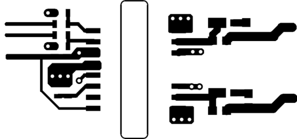
Figure 9-2. Top Layer Traces and Copper
