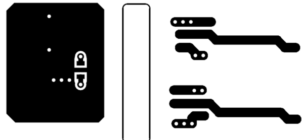
Figure 9-3. Bottom Layer Traces and Copper
