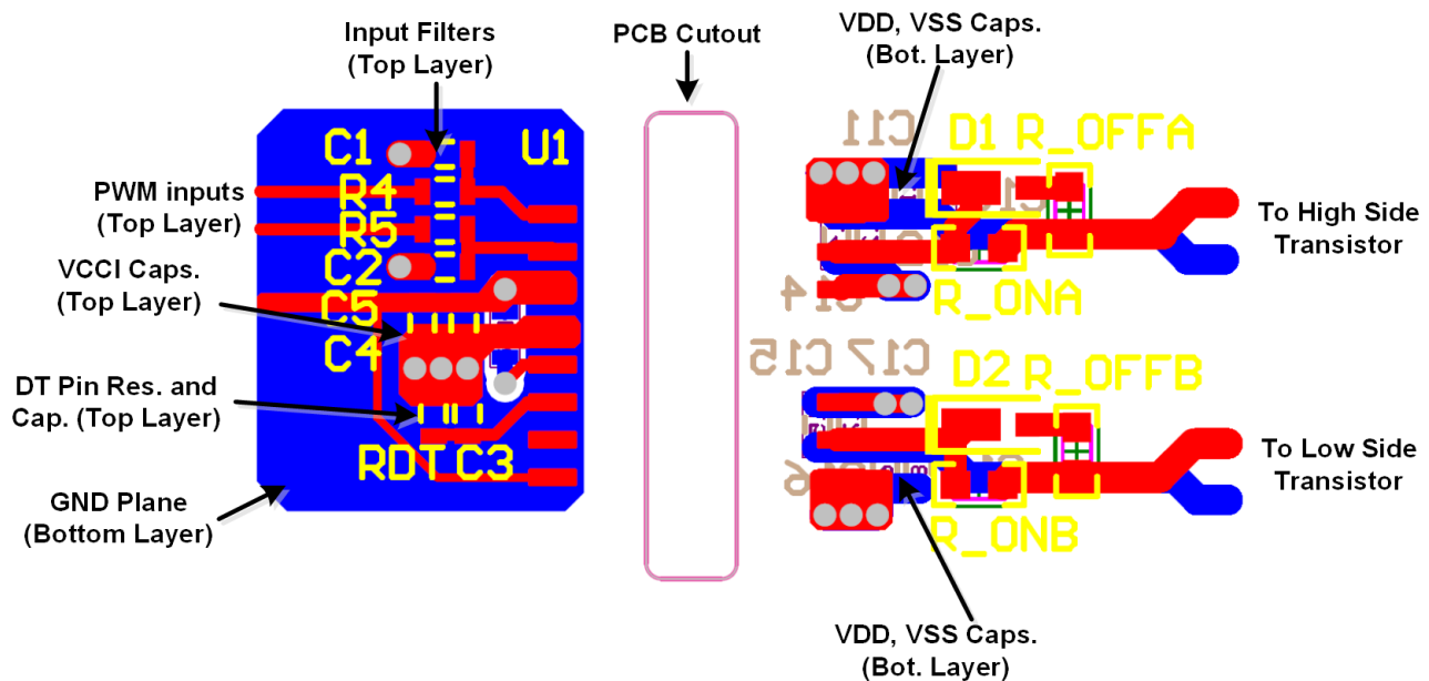
Figure 9-1. Layout Example
