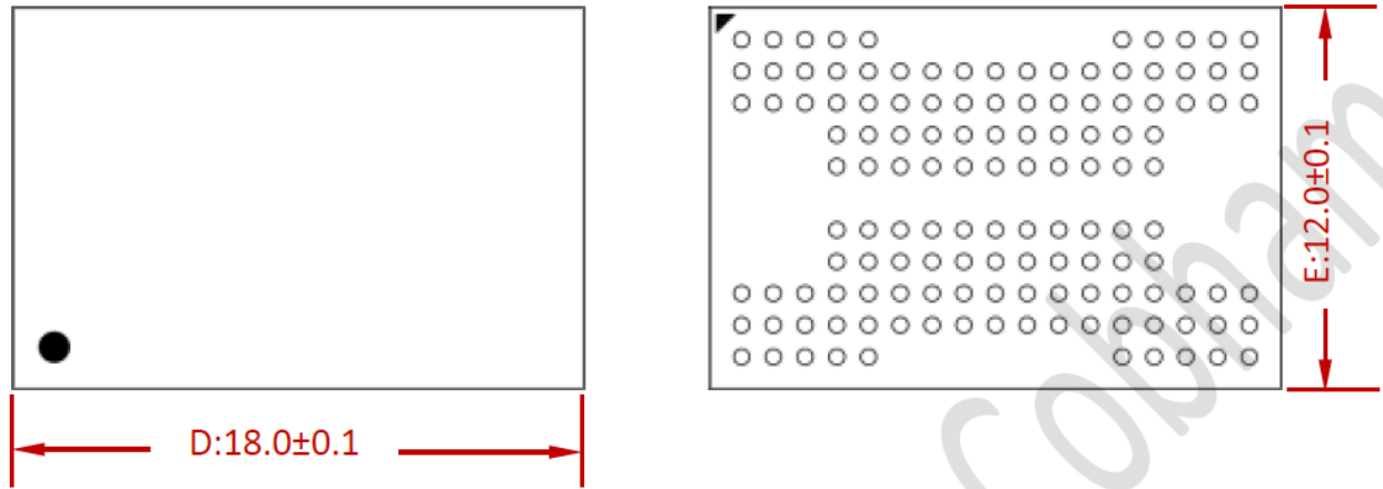
Figure 2: 132-Ball LPGA - 12mm x 18mm
