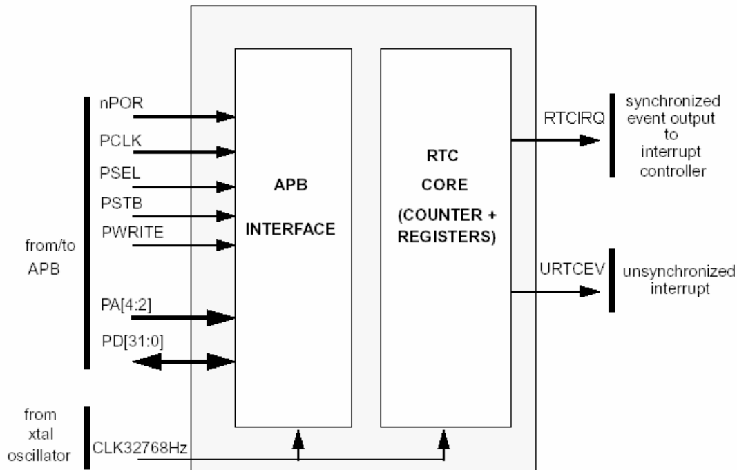
Figure 10-6 RTC Connection
