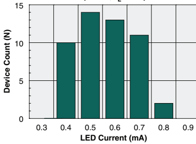
Typical I F for Switch Operation (N=50, I L =120)
