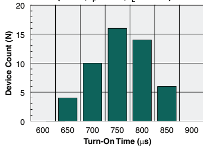
Typical Turn-On Time Distribution (N=50, I F =5mA, I L =60mA)
