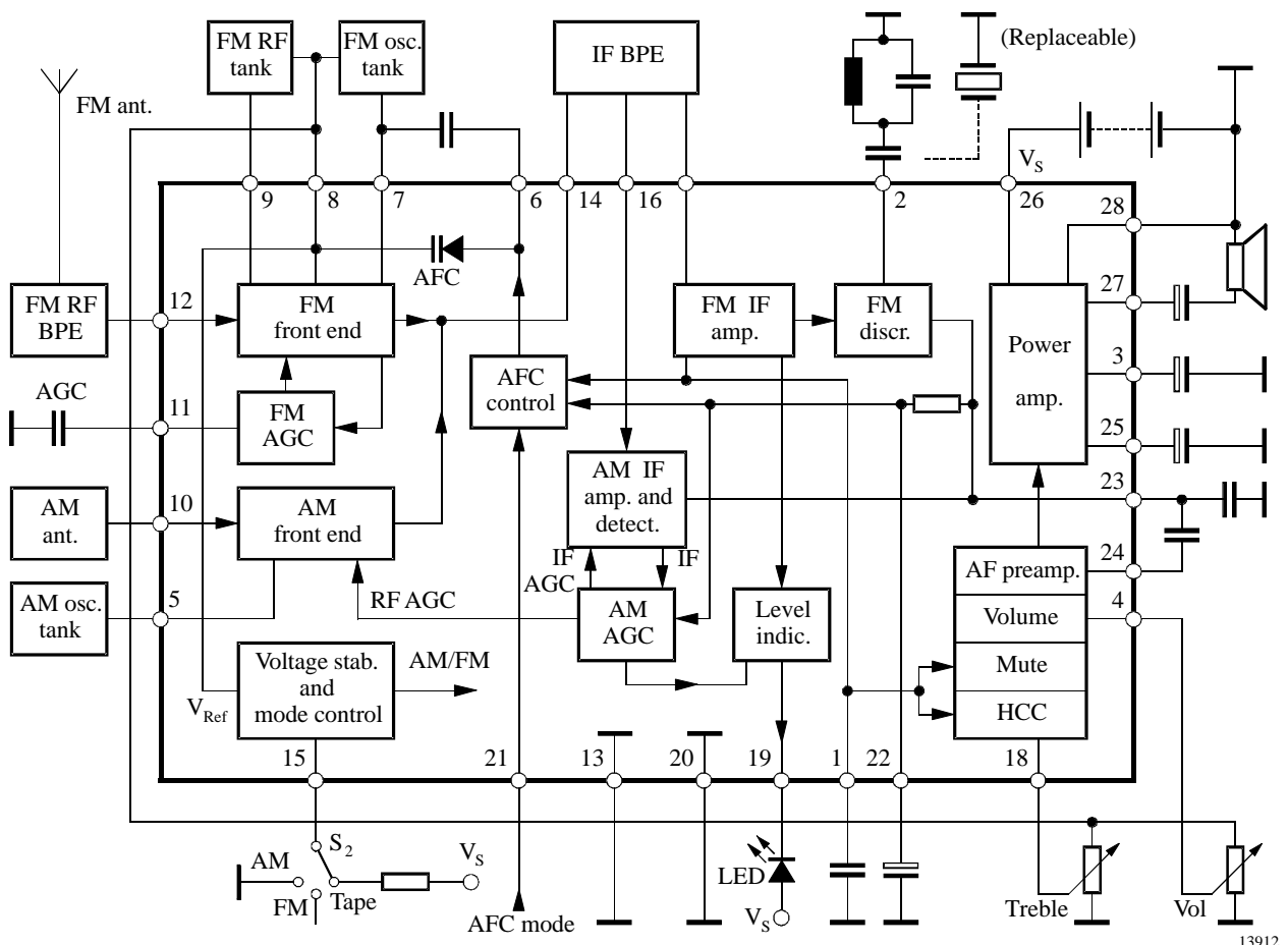
Figure 1. Block diagram
