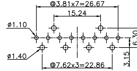
PC Board Layout Component Side Shown
