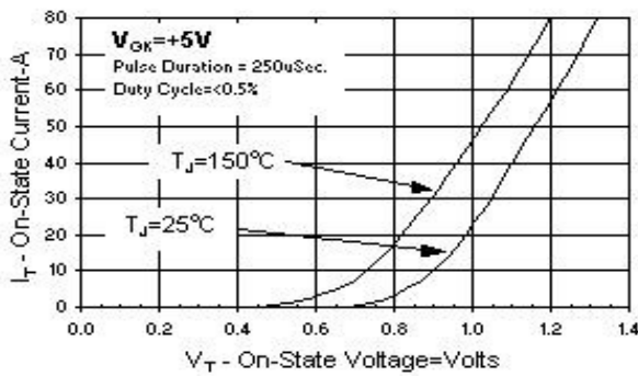
Figure 1. On-State Characteristics
