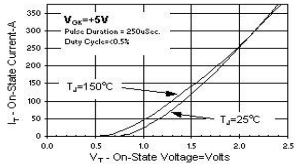
Figure 2. On-State Characteristics
