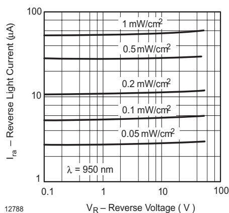
Figure 5. Reverse Light Current vs. Reverse Voltage
