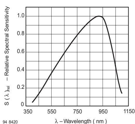
Figure 7. Relative Spectral Sensitivity vs. Wavelength
