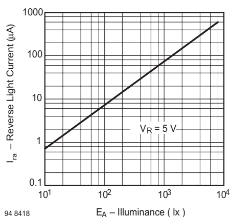
Figure 4. Reverse Light Current vs. Illuminance
