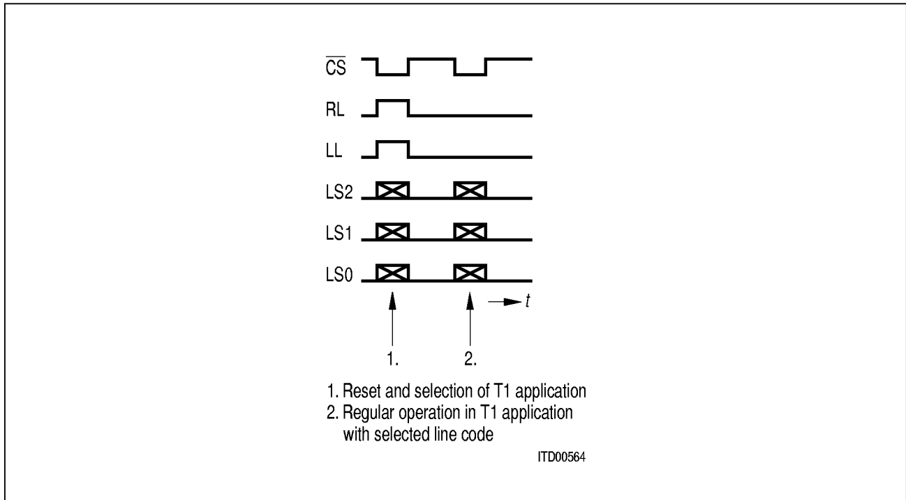
Figure 10 Timing of Software Programming for T1 Application
