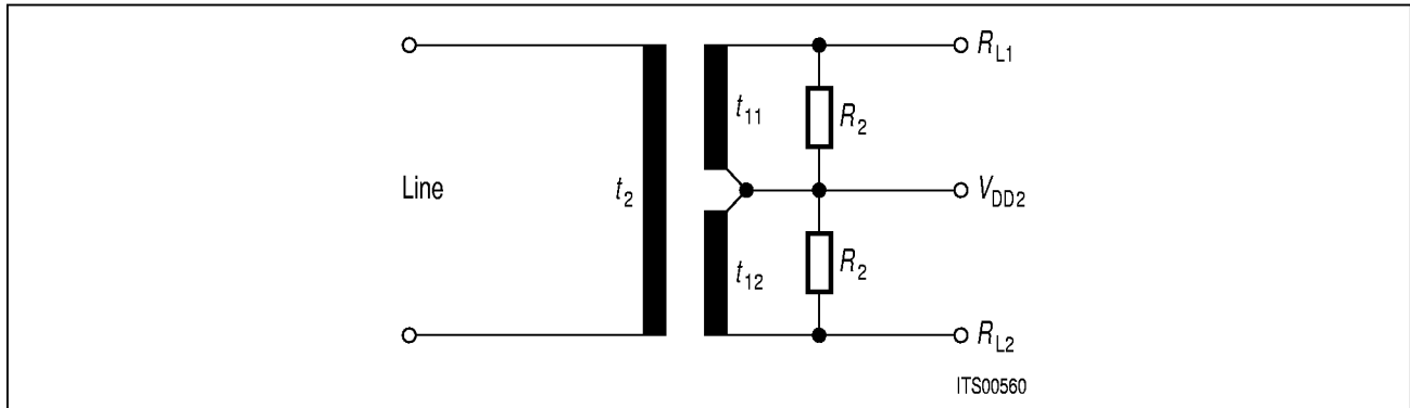
Figure 6 Receiver Configuration
