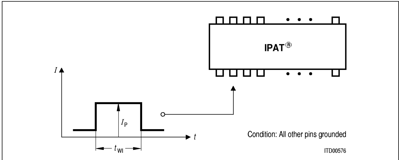
Figure 21 Measurement of Overvoltage Stress
