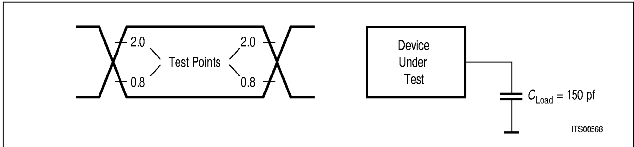
Figure 13 Input/Output Waveform for AC Tests
