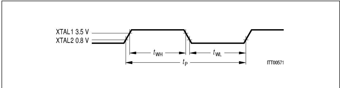
Figure 16 Timing of XTAL1/XTAL2
