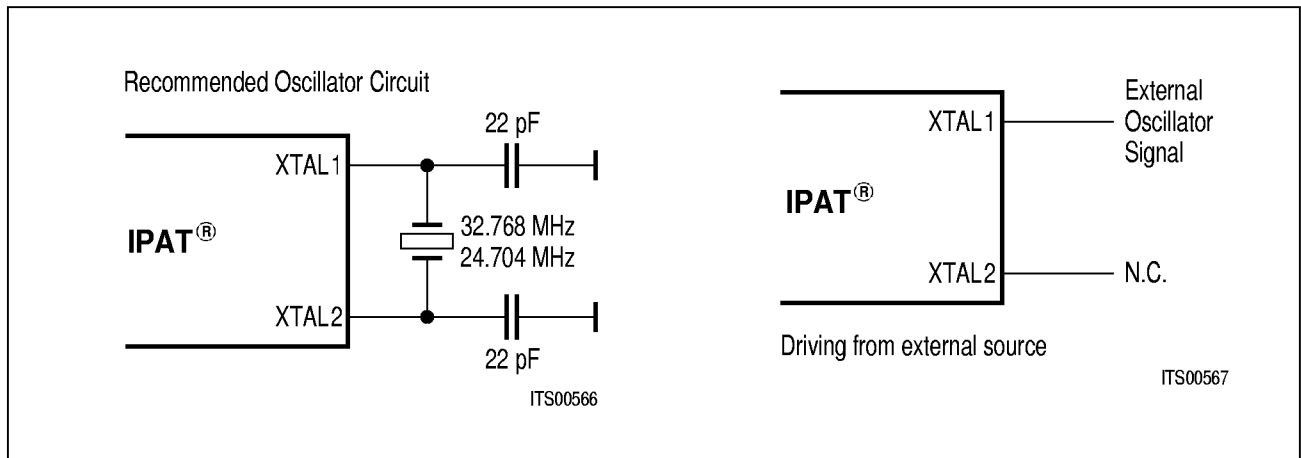
Figure 12 Oscillator Circuits
