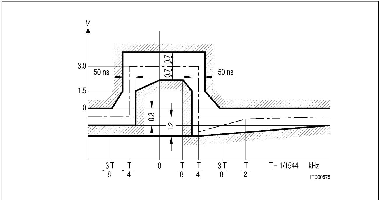
Figure 20 Pulse Shape at NTT Interface
