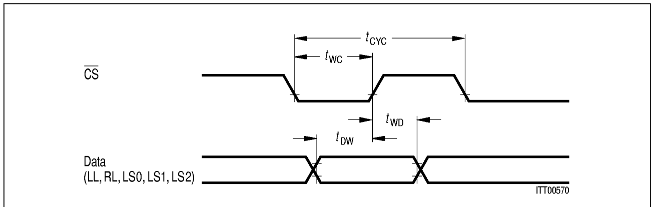
Figure 15 Timing of the Microprocessor Interface
