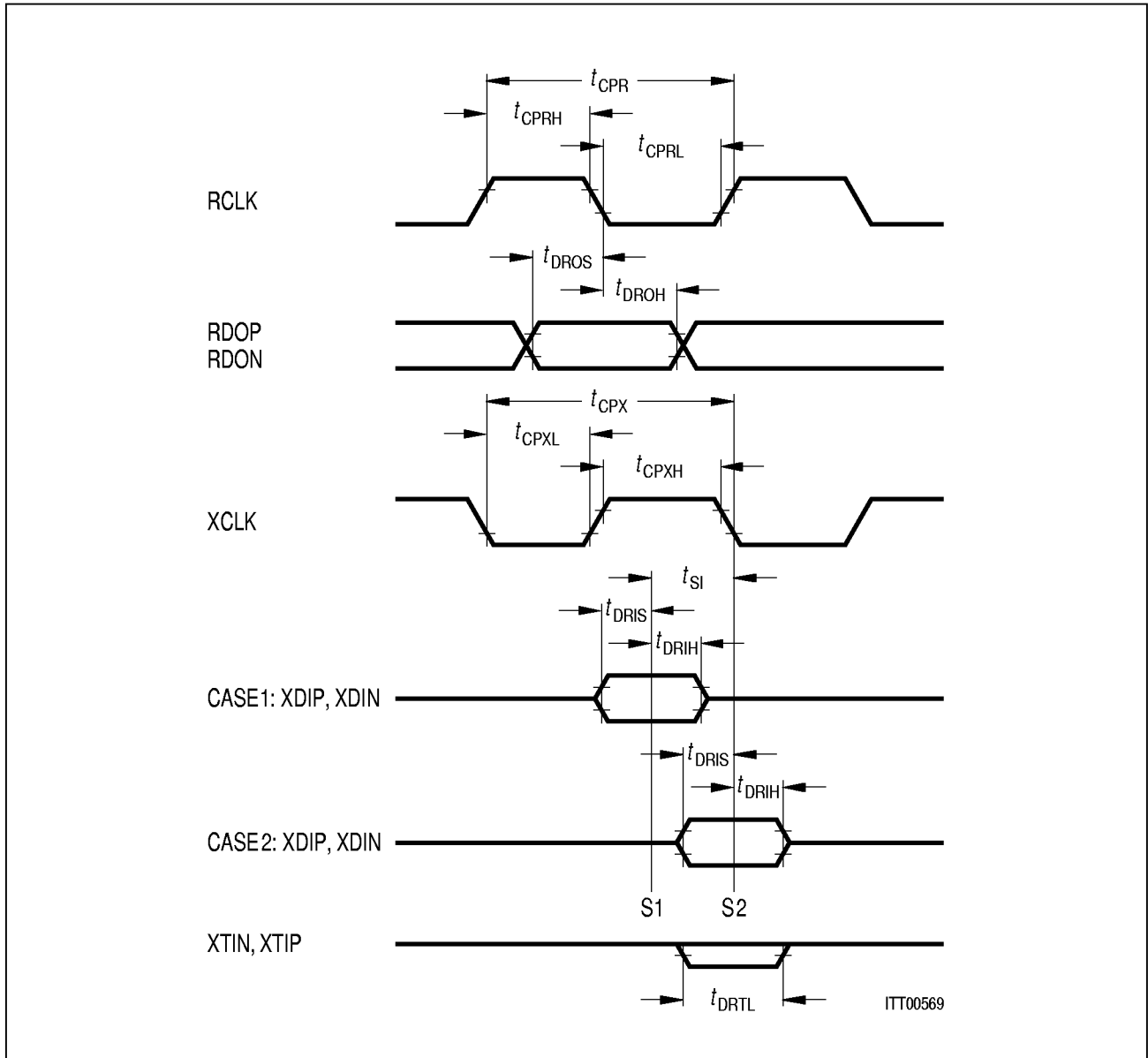
Figure 14 Timing of the Dual Rail Interface
