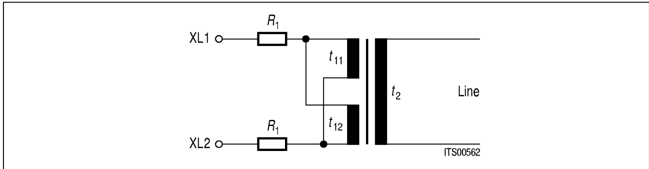
Figure 8 Transmitter Configuration
