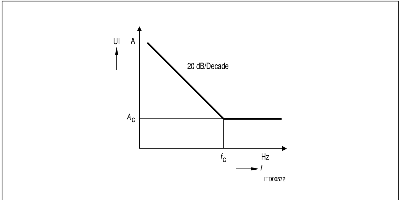
Figure 17 IPAT® Receive Jitter Tolerance
