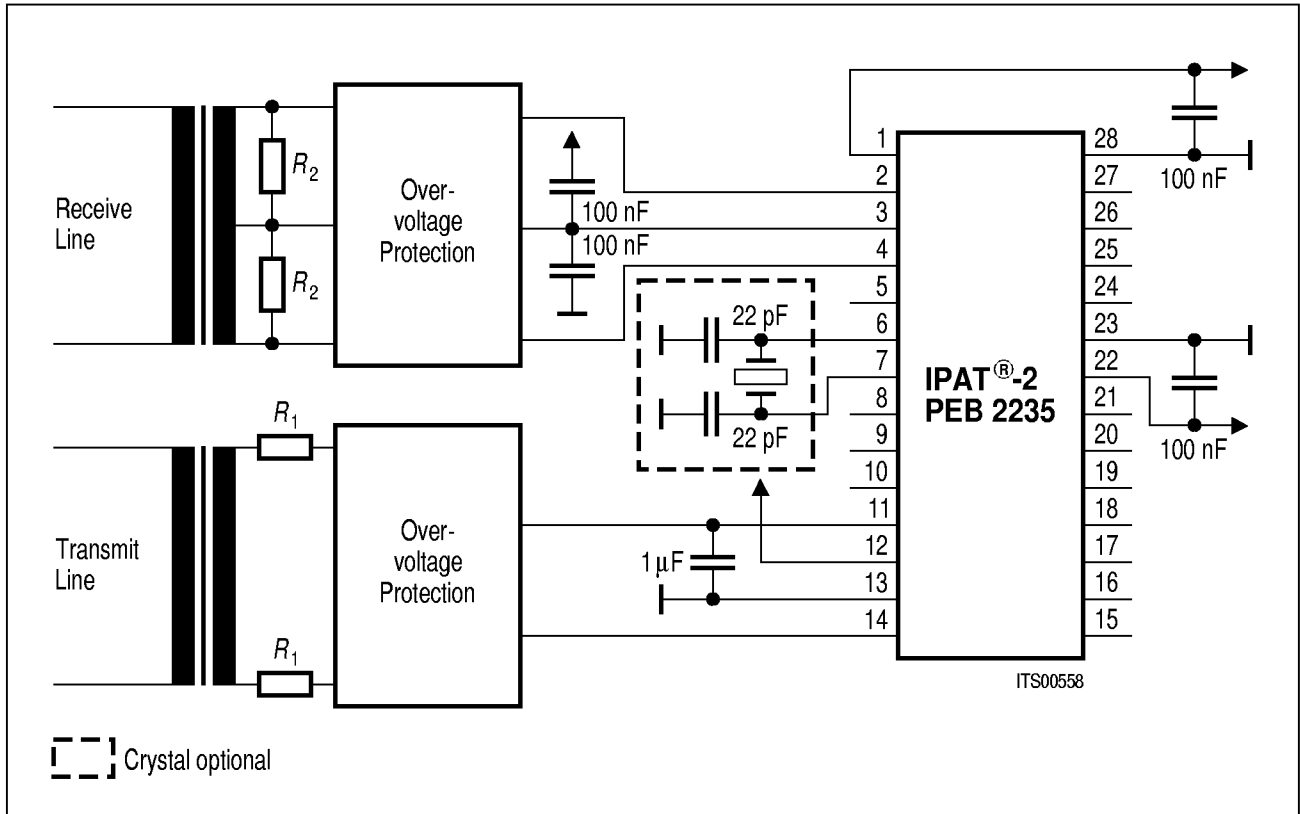
Figure 2 External Wiring of the IPAT®
