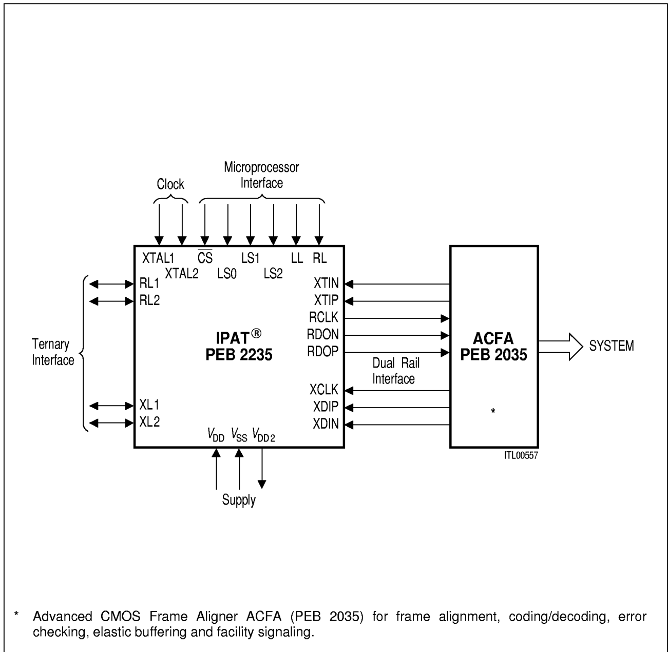
Figure 1 Logic Diagram of the IPAT ®
