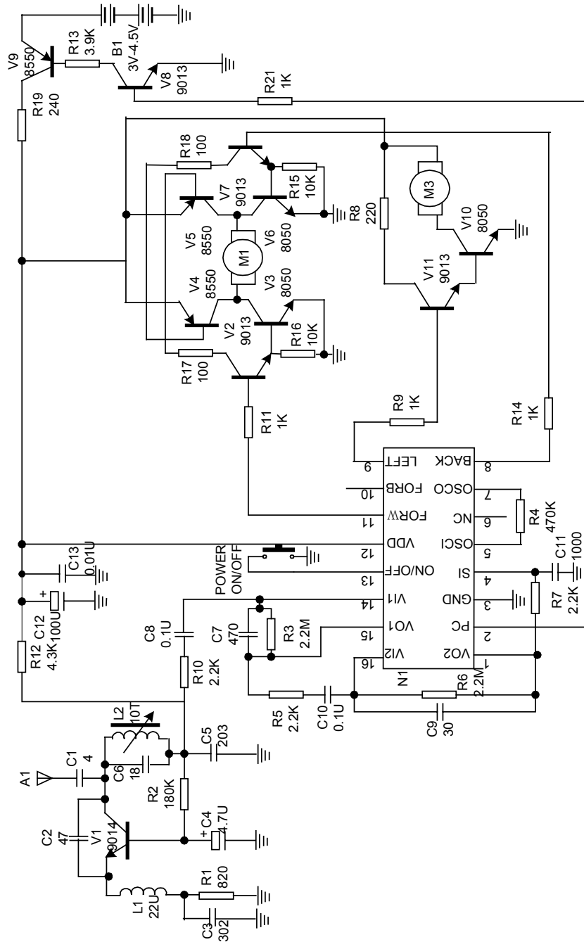
Figure 5 APPLICATION CIRCUIT(3-4.5V)
