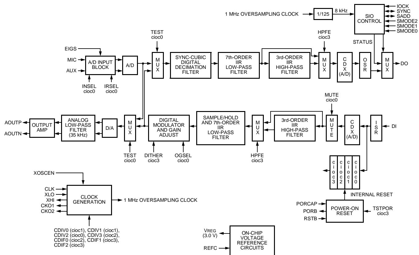
Figure 3. CSP1027 Block Diagram
