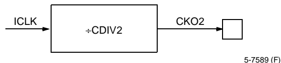
Figure 18. Clock Divider 2
