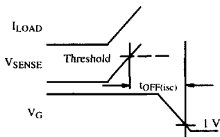
Figure 6. First Short Circuit
