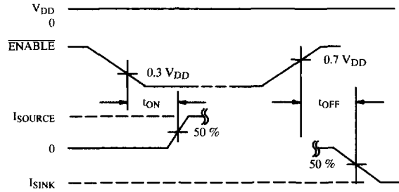
Figure 3. Normal-Mode Operation
