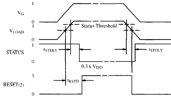
Figure 8. \overline{STATUS} and \overline{RESET}
