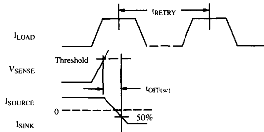
Figure 7. Relaxation-Mode Current Limit
