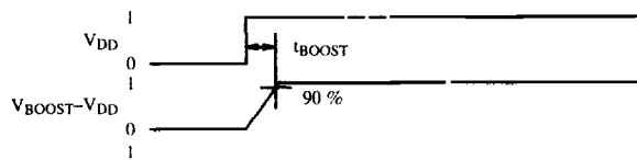
Figure 5. Start of Boost Converter
