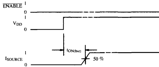
Figure 4. Timing Definition with \overline{\text{ENABLE}} Already On
