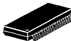
Outline 36P2R-A 0.8mm pitch 450mil SSOP (8.4mmx15.0mmx2.0mm)
