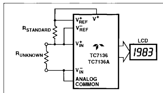
Figure 12 Low Parts Count Ratiometric Resistance Measurement
