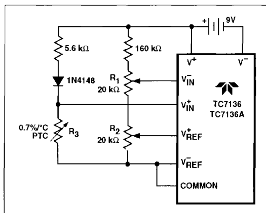
Figure 14 Positive Temperature Coefficient Resistor Temperature Sensor
