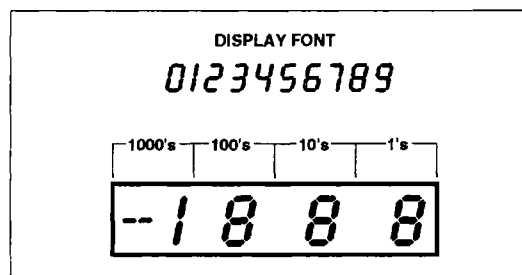
Figure 6 Display FONT and Segment Assignment
