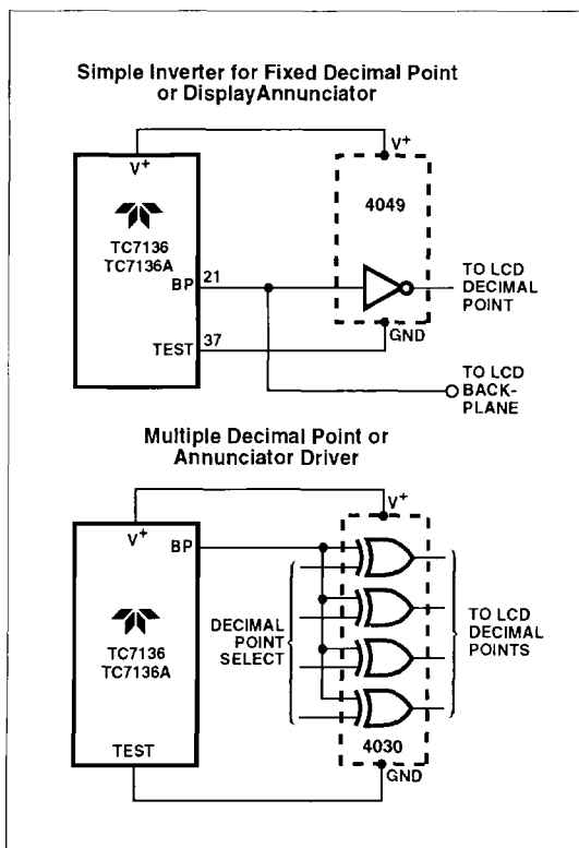
Figure 11 Decimal Point and Annunciator Drives
