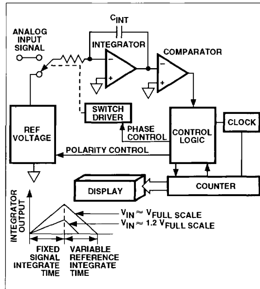
Figure 1 Basic Dual-Slope Converter
