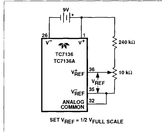
Figure 10 TC7136A Internal Voltage Reference Connection
