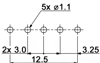
HOLE LAYOUT TOP VIEW \oplus 0.05
