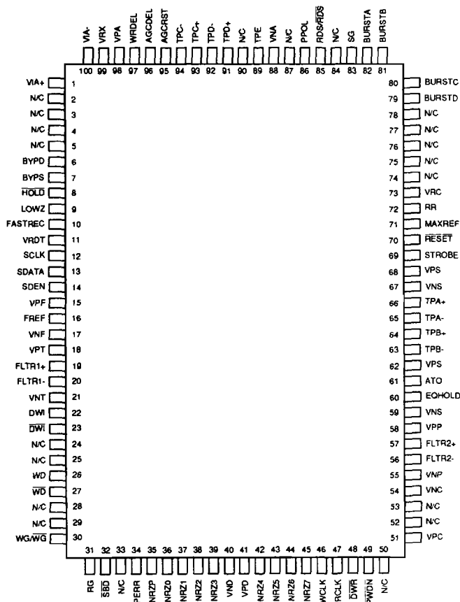
100-Lead QFP
