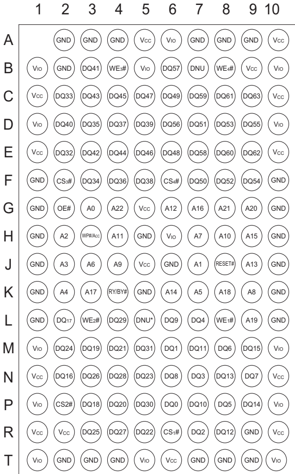
FIG 1: PIN CONFIGURATION FOR W78M64VP-XSBX (TOP VIEW)
