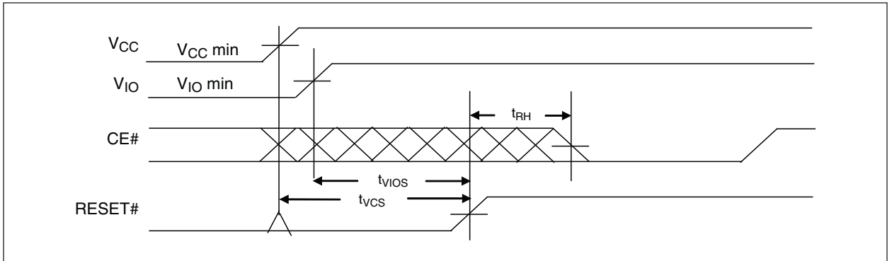
FIG. 19: POWER-UP SEQUENCE TIMINGS
