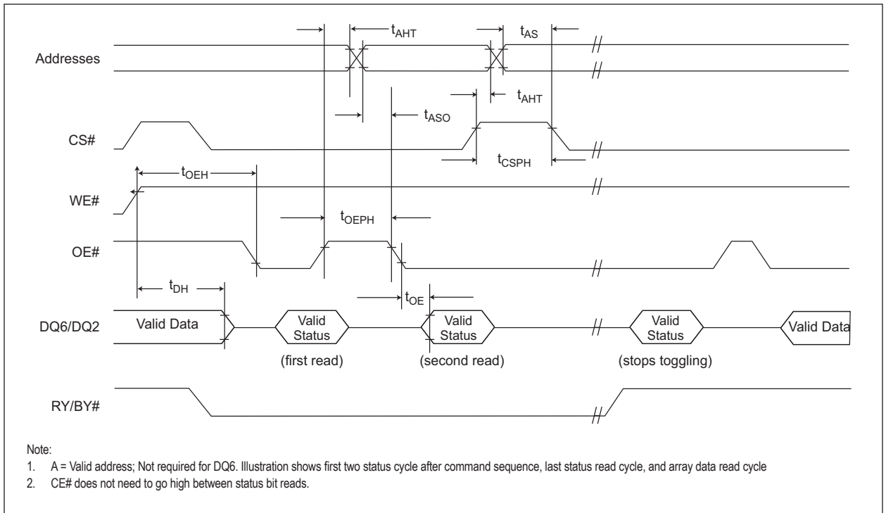
FIG 24: TOGGLE BIT TIMINGS (DURING EMBEDDED ALGORITHMS)
