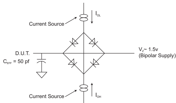
FIG. 14 AC TEST CIRCUIT
