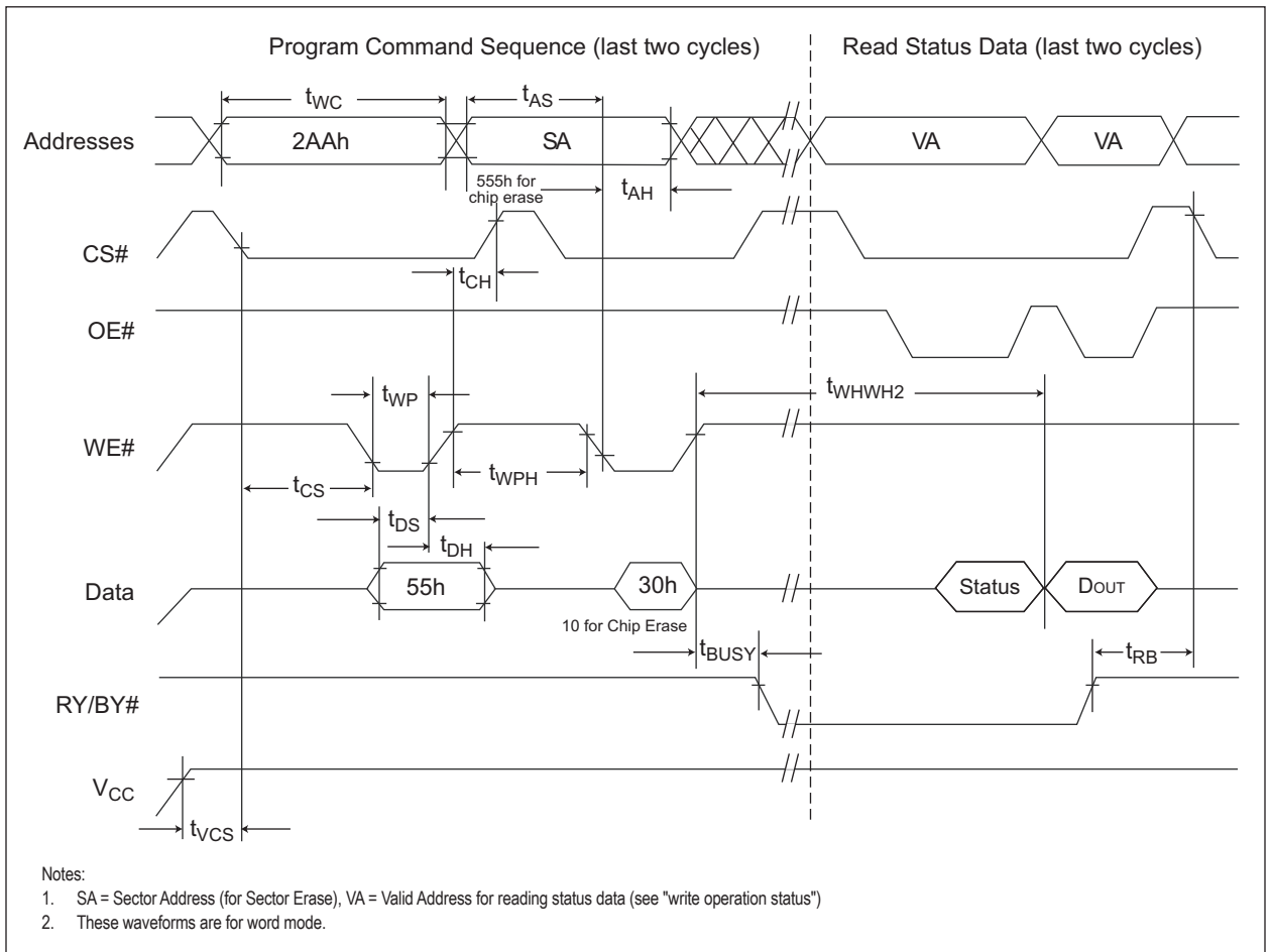
FIG 22: CHIP/SECTOR ERASE OPERATION TIMINGS
