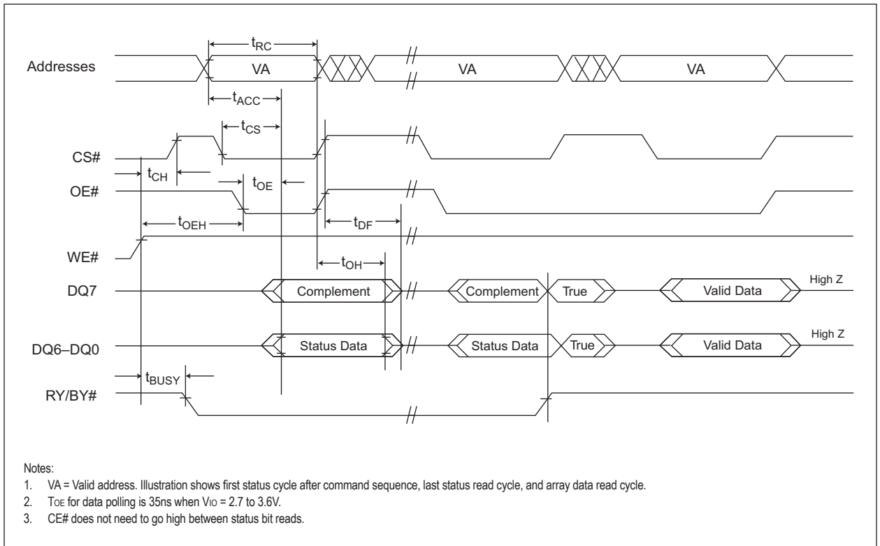
FIG 23: DATA# POLLING TIMINGS (DURING EMBEDDED ALGORITHMS)
