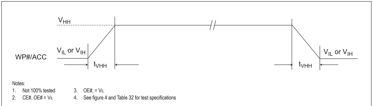
FIG 21: ACCELERATED PROGRAM TIMING DIAGRAM
