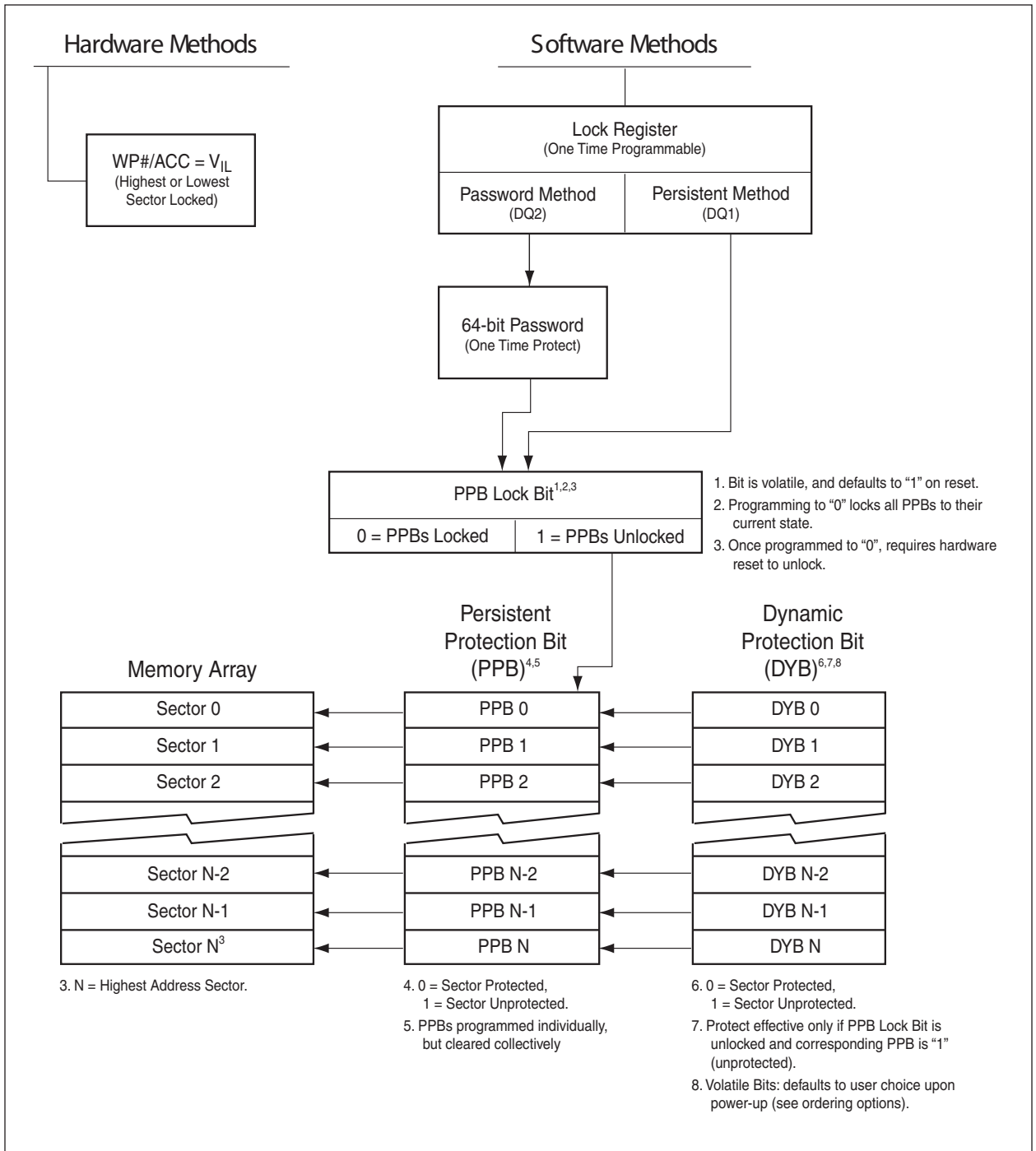
FIG: 9 ADVANCED SECTOR PROTECTION/UNPROTECTION
