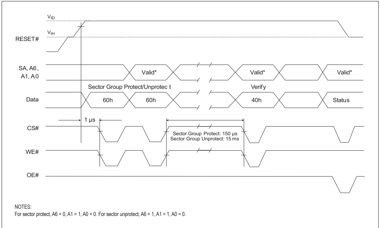
FIG 26: SECTOR/SECTOR BLOCK PROTECT AND UNPROTECT TIMING DIAGRAM
