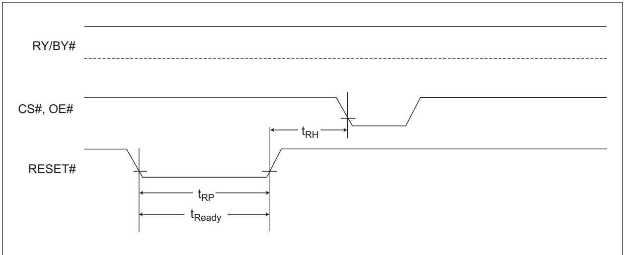
FIG. 17: RESET TIMINGS NOT DURING EMBEDDED ALGORITHMS
