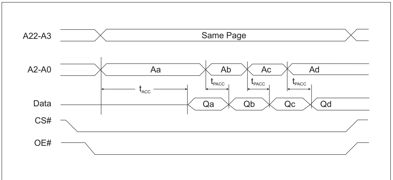
FIG 16: PAGE READ OPERATION TIMINGS
