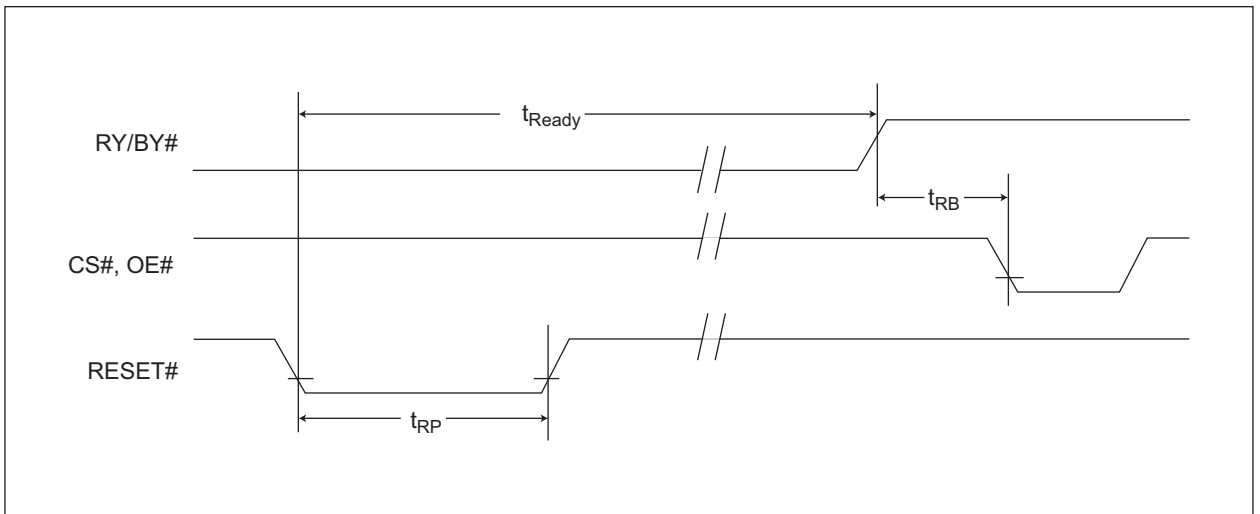
FIG. 18: RESET TIMINGS DURING EMBEDDED ALGORITHMS
