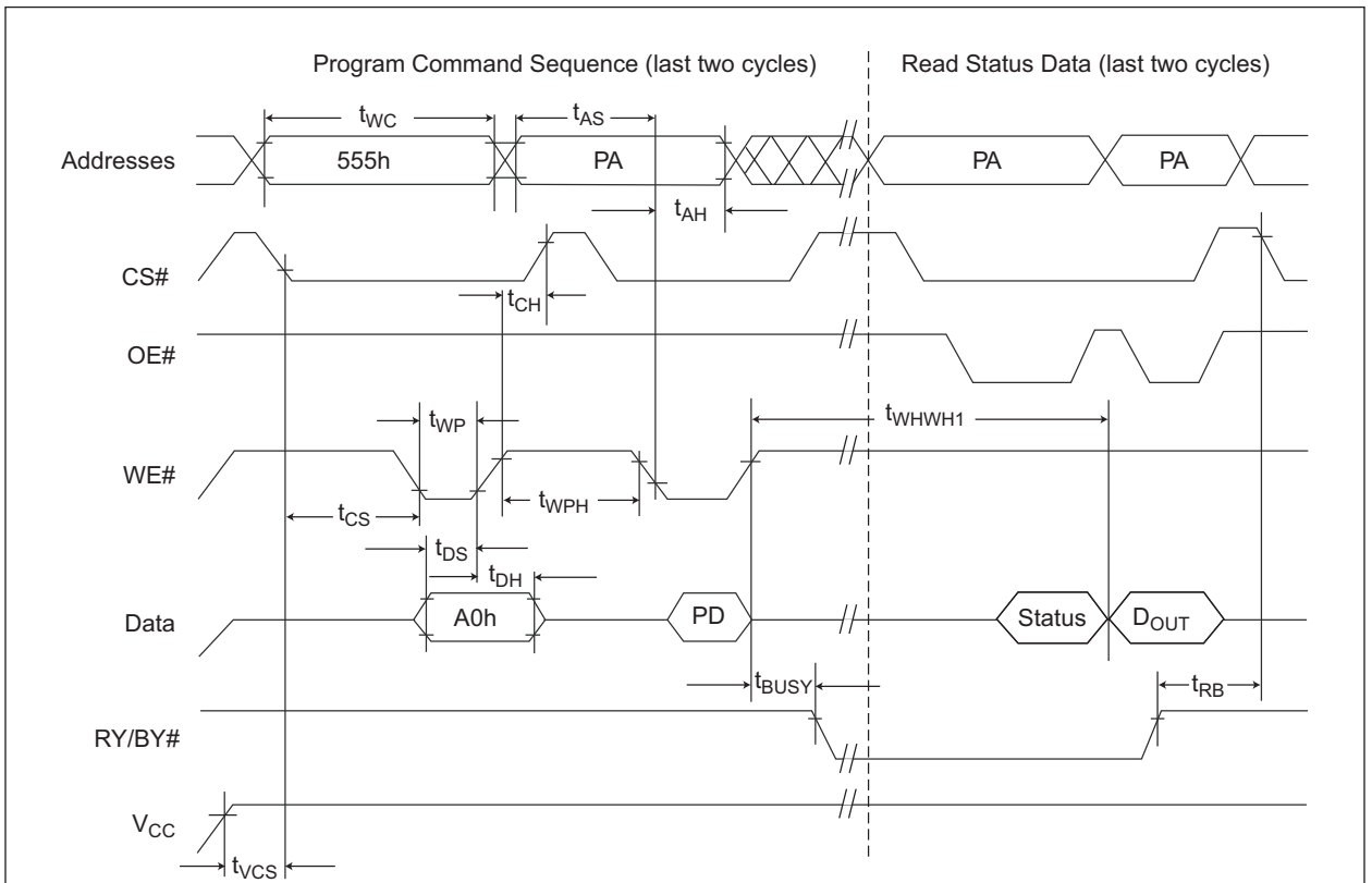
FIG. 20: PROGRAM OPERATION
