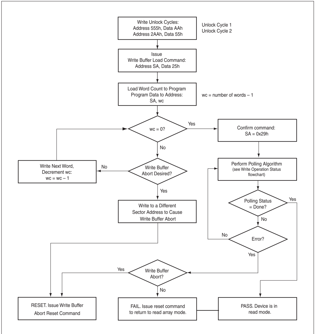
FIG: 6 WRITE BUFFER PROGRAMMING OPERATION
