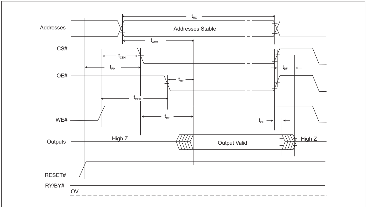
FIG 15: AC WAVEFORMS FOR READ OPERATIONS
