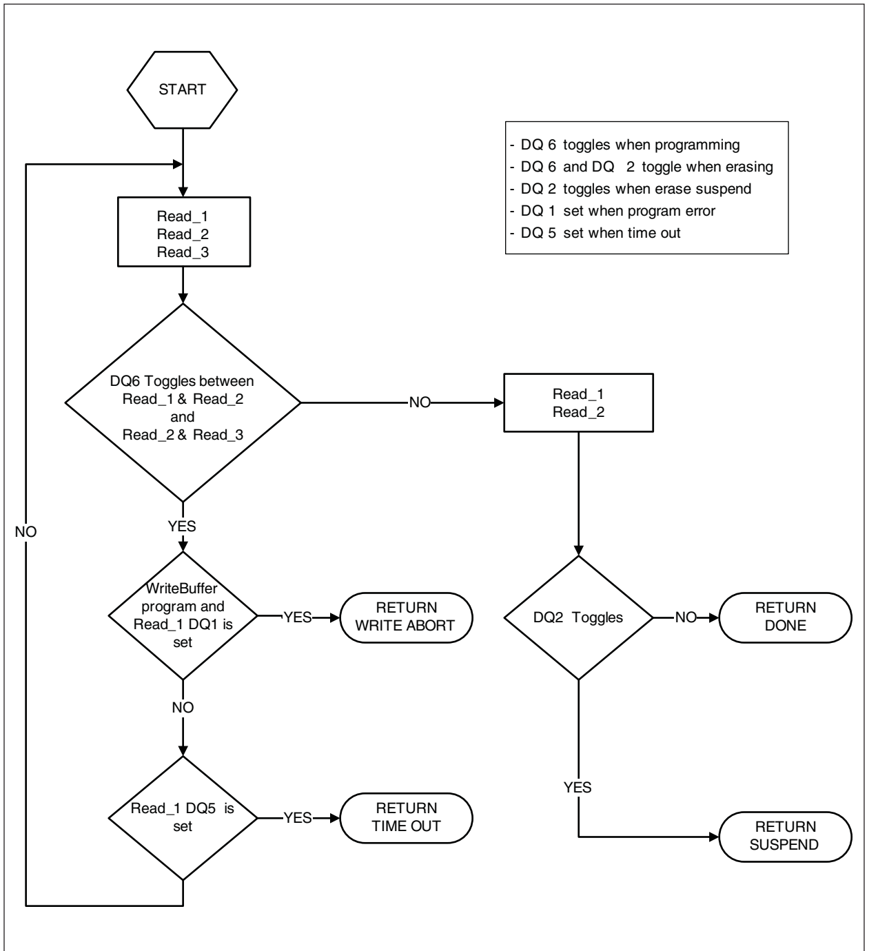
FIG: 8 WRITE OPERATION STATUS FLOWCHART
