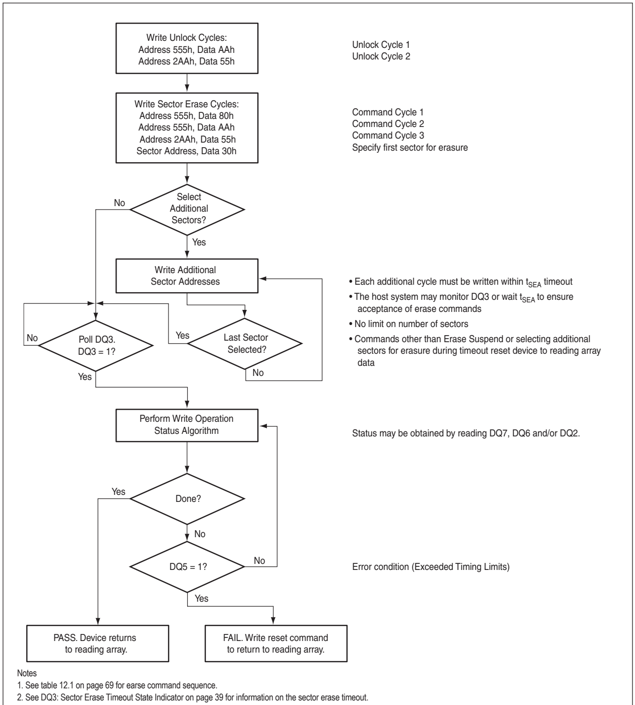
FIG: 7 SECTOR ERASE OPERATION
