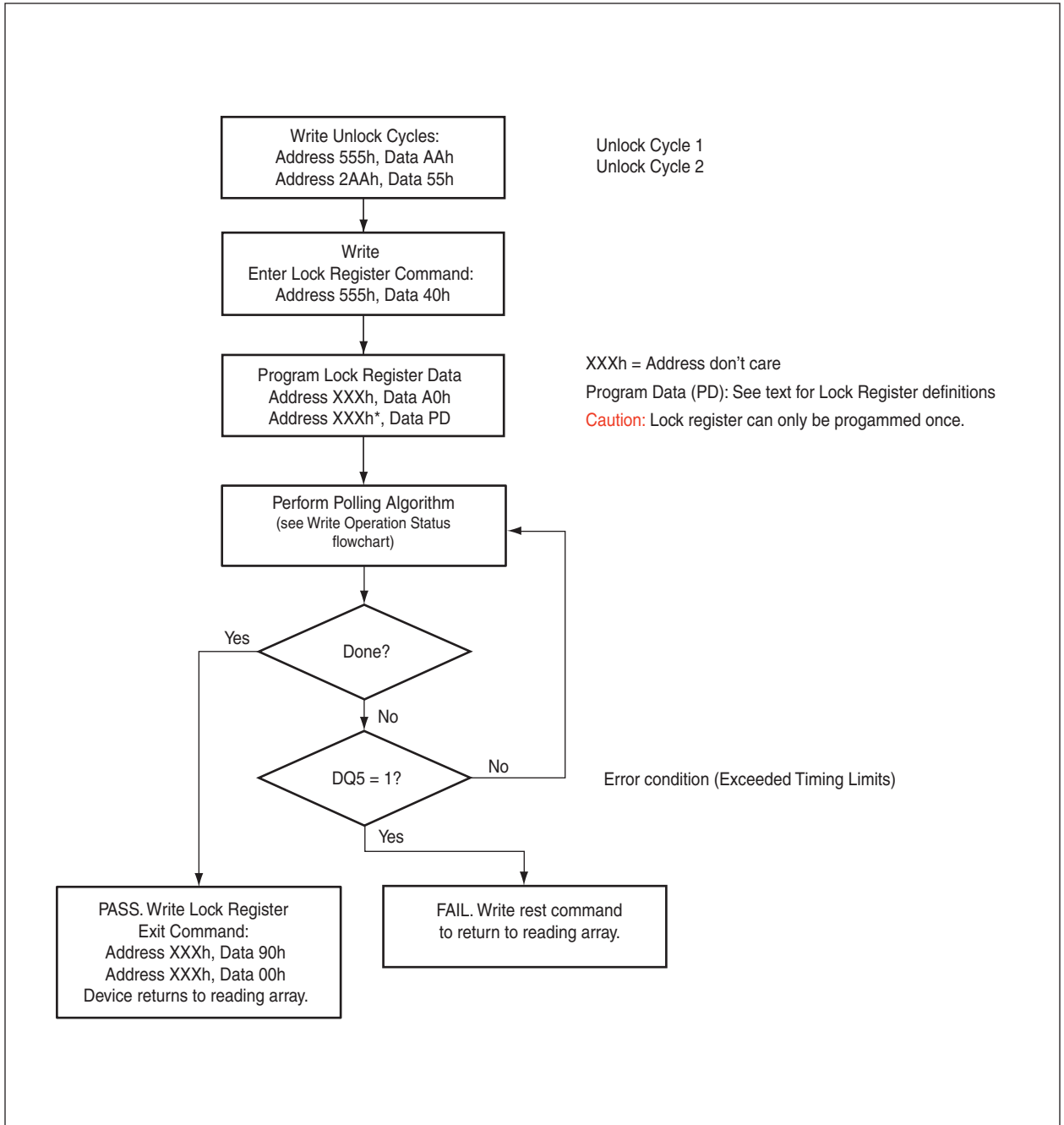
FIG: 11 LOCK REGISTER PROGRAM ALGORITHM
