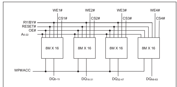
FIG 3: BLOCK DIAGRAM
