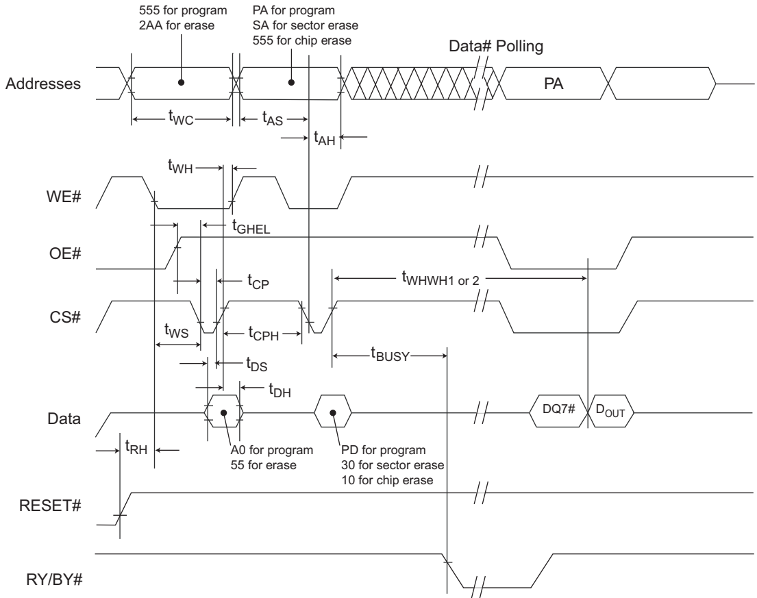
FIG 27: ALTERNATE CS# CONTROLLED WRITE (ERASE/PROGRAM) OPERATION TIMINGS
