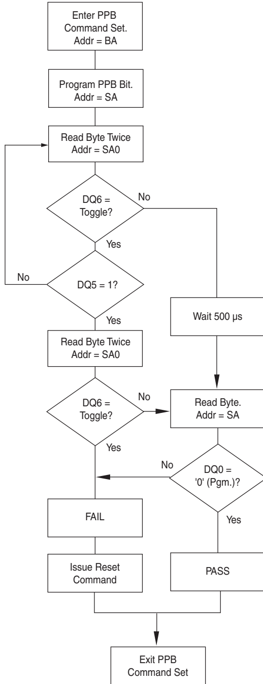
FIG: 10 PPB PROGRAM ALGORITHM
