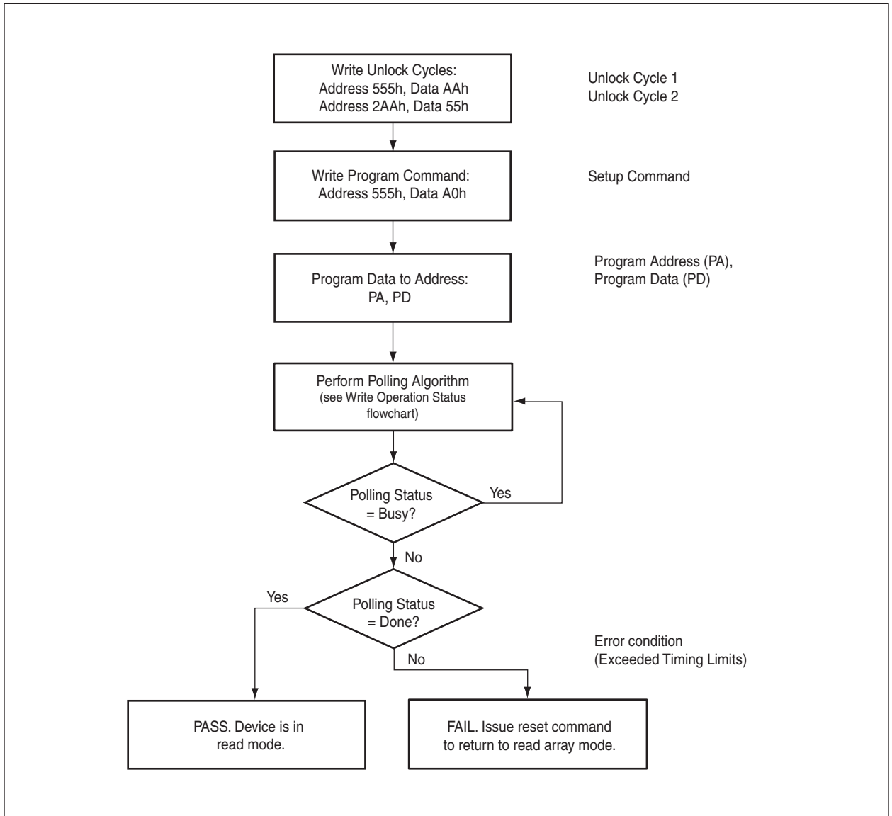
FIG: 5 SINGLE WORD PROGRAM
