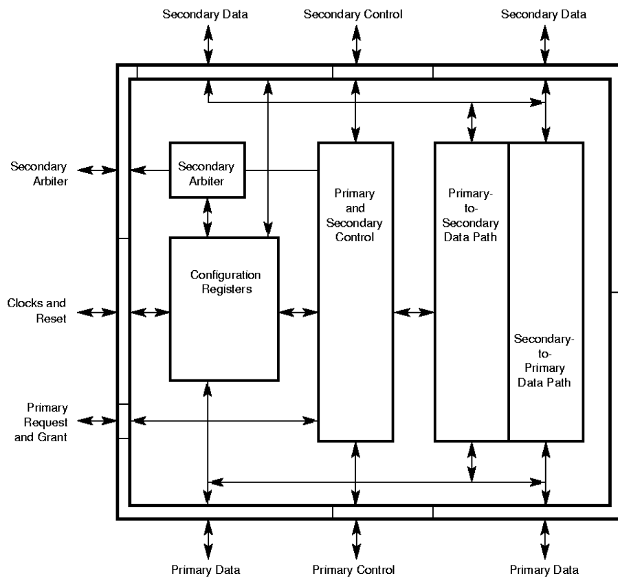
Figure 1-3. 21152 Block Diagram
