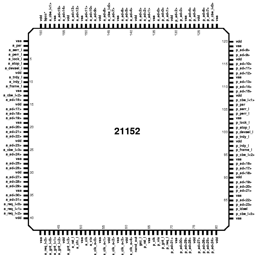
Figure 3-1. 21152 Pinout Diagram
