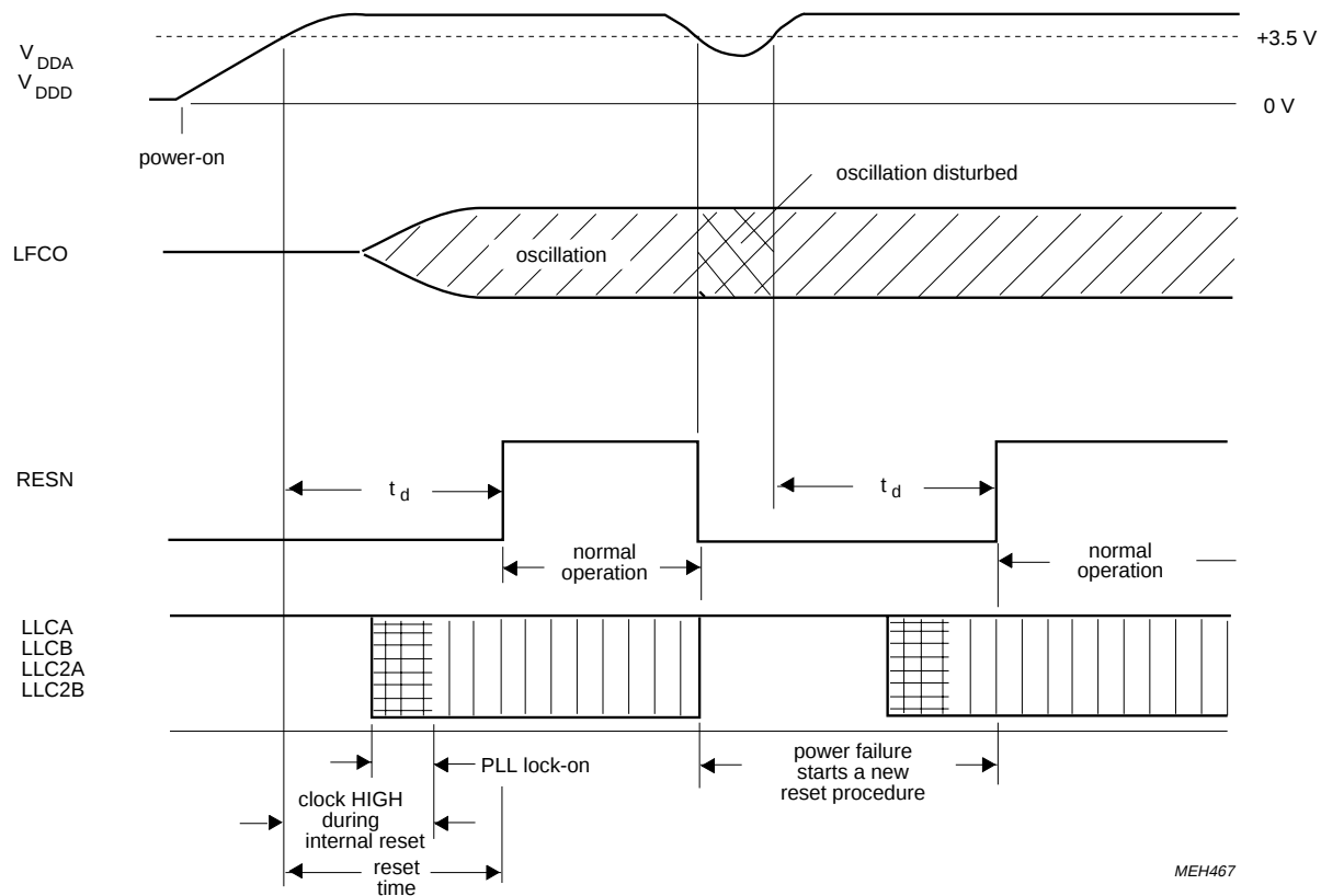
Fig.4 Reset procedure.
