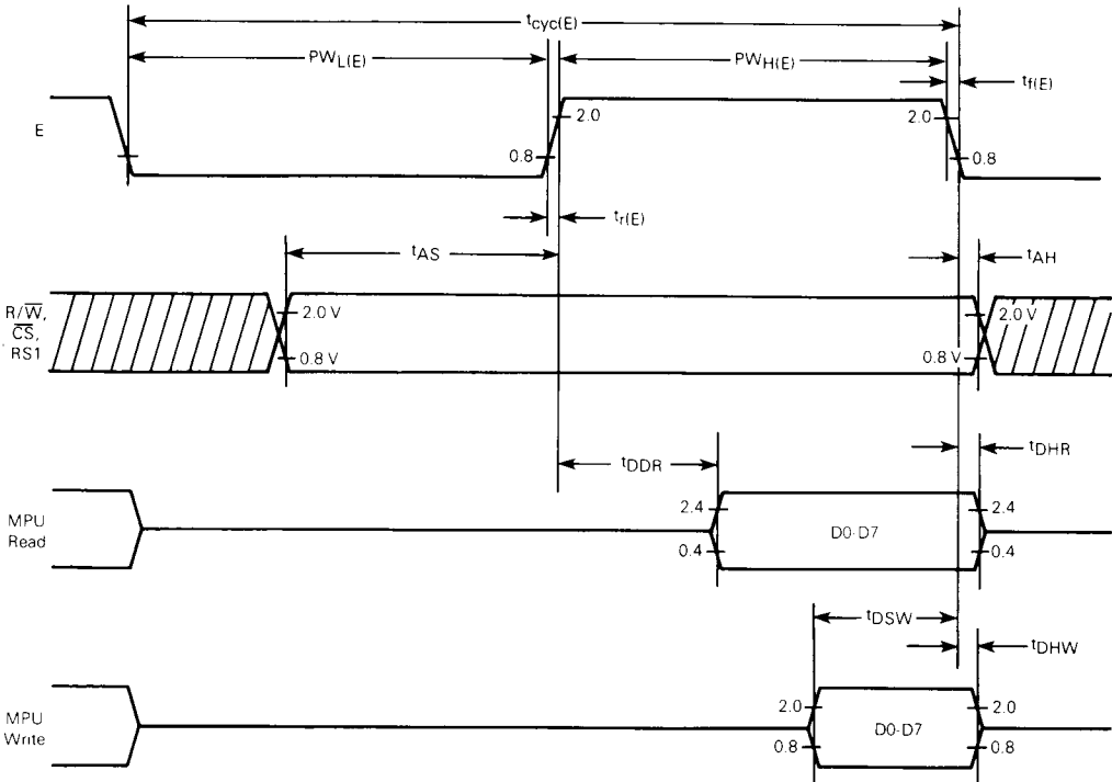
FIGURE 1 — BUS TIMING
