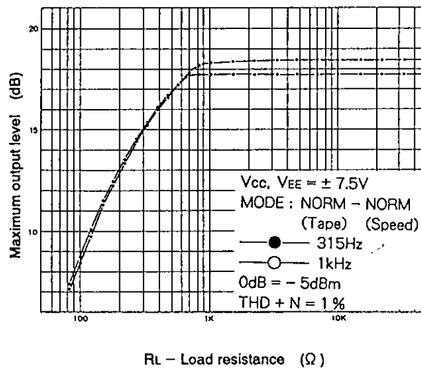
Load characteristics
