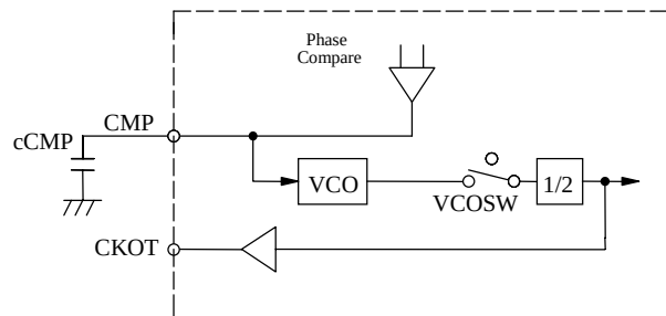
Figure5 VCO
