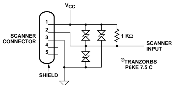
Figure 6. Recommended Interface.
