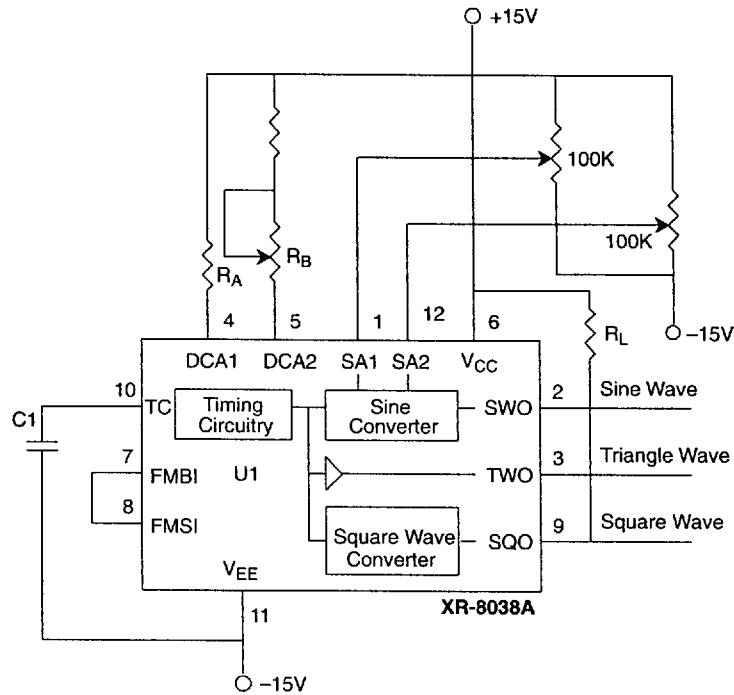
Figure 7. Minimum Sine Wave Distortion
