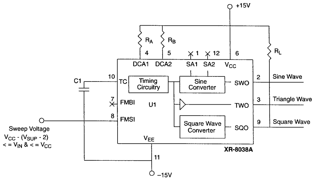
Figure 9. Frequency Sweep
