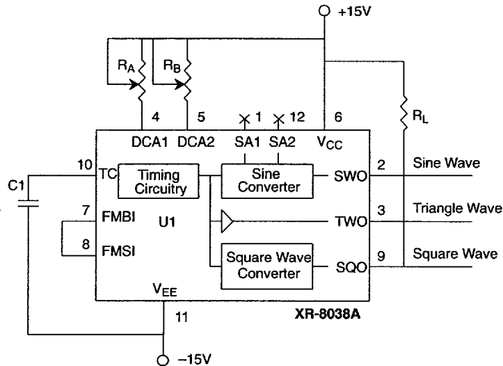
Figure 4. Possible Connection for External Duty Cycle Adjust
