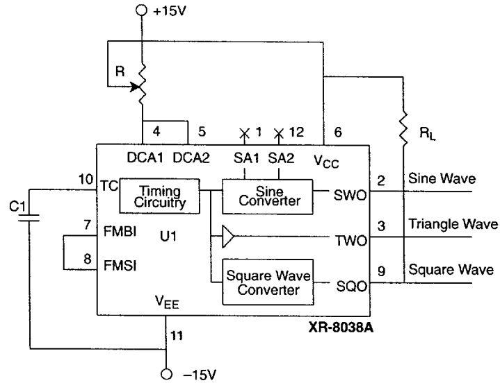
Figure 6. No Duty Cycle Adjust
