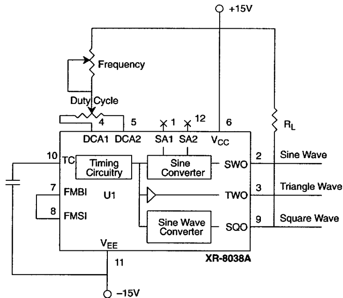
Figure 5. Single Potentiometer for External Duty Cycle Adjust
