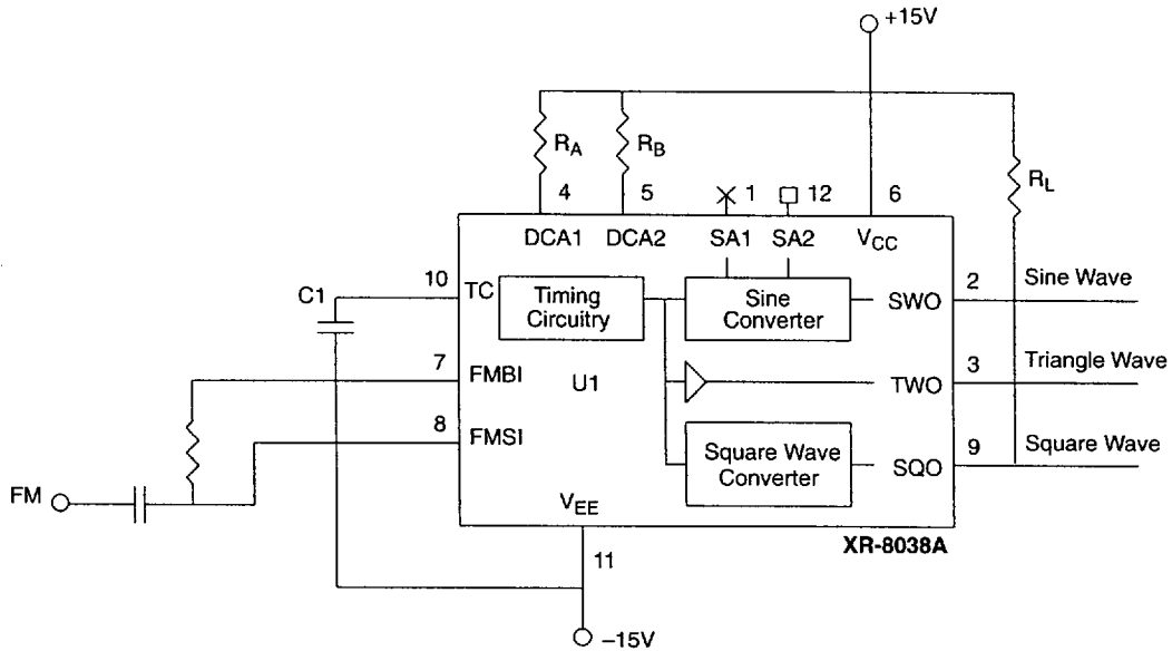
Figure 8. Frequency Modulator
