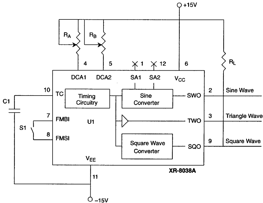
Figure 2. Generalized Test Circuit
