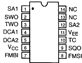
14 Lead PDIP (0.300")
