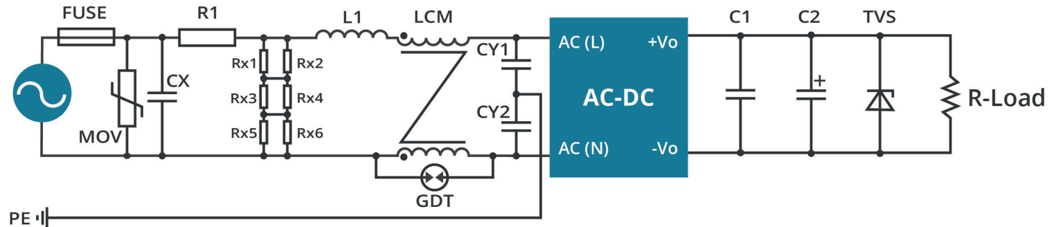
Figure 3 RECCOMENDED CIRCUIT FOR CLASS I EQUIPMENT
