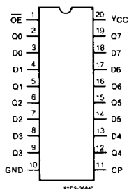
CD54/74AC/ACT374
