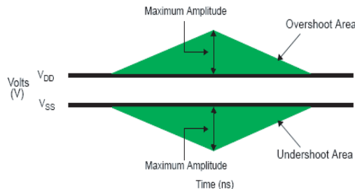
Address and Control Overshoot and Undersheet Definition
