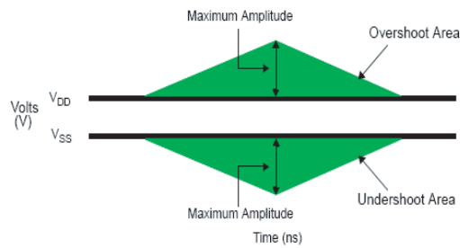
Clock, Data, Strobe, Mask Overshoot and Undersheet Definition
