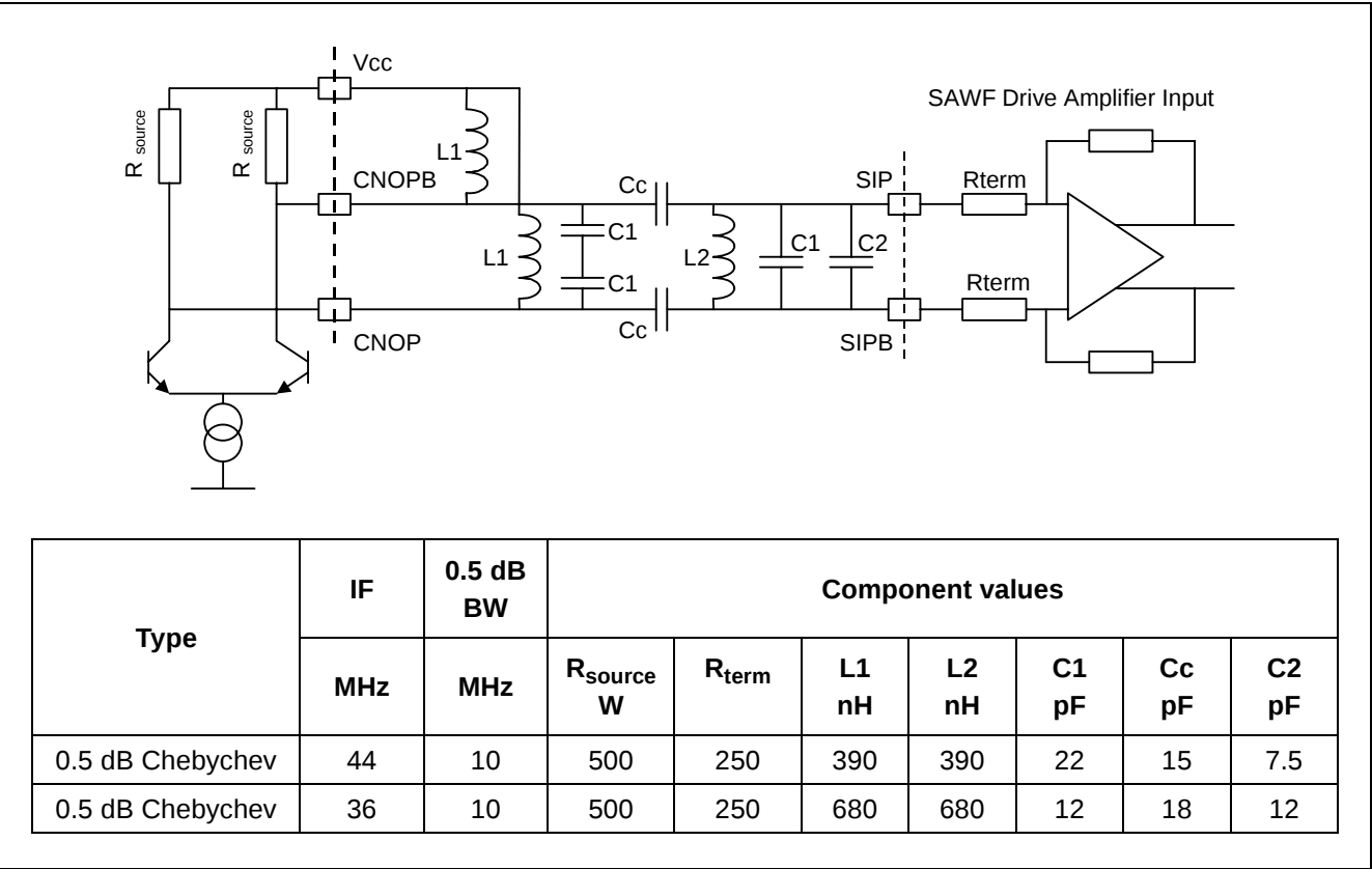
Figure 11 - Interstage Filter
