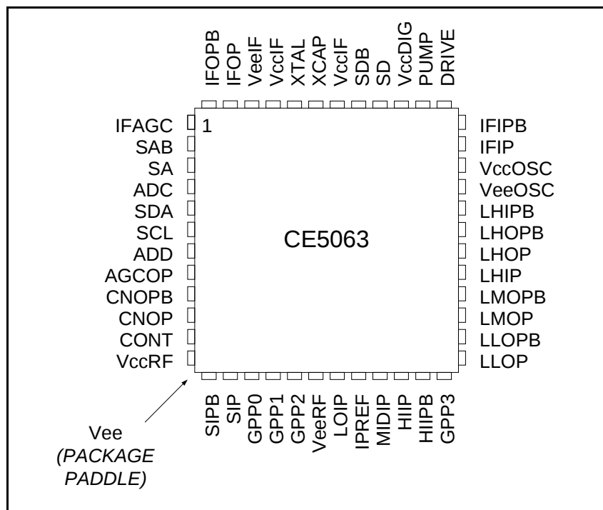
Figure 2 - Pin Diagram
