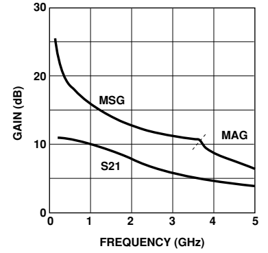
Figure 19. AT-30511 Gains vs. Frequency at V_{CE} = 2.7 V, I_C = 1 mA.
