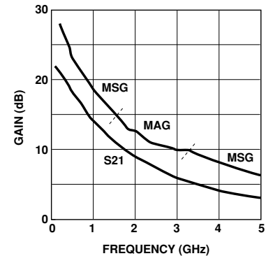
Figure 20. AT-30533 Gains vs. Frequency at V_{CE} = 2.7 V, I_C = 1 mA.
