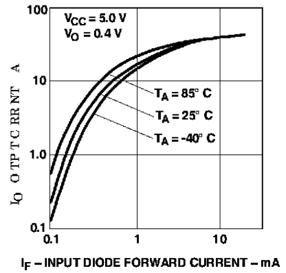
Figure 3. Output Current vs. Input Diode Forward Current.
