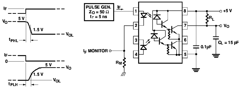
Figure 9. Switching Test Circuit.
