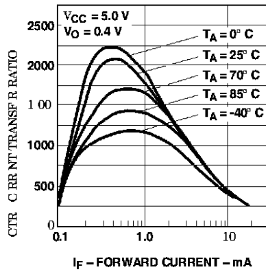
Figure 2. Current Transfer Ratio vs. Forward Current.
