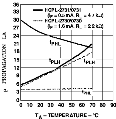
Figure 7. Propagation Delay vs. Temperature.
