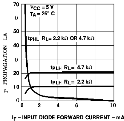
Figure 8. Propagation Delay vs. Input Diode Forward Current.
