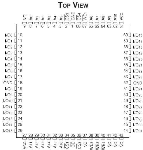
Fig. 3 PIN CONFIGURATION FOR WE128K32-XG2UX, WE128K32-XG1UX 1 AND WE128K32-XG1TX
