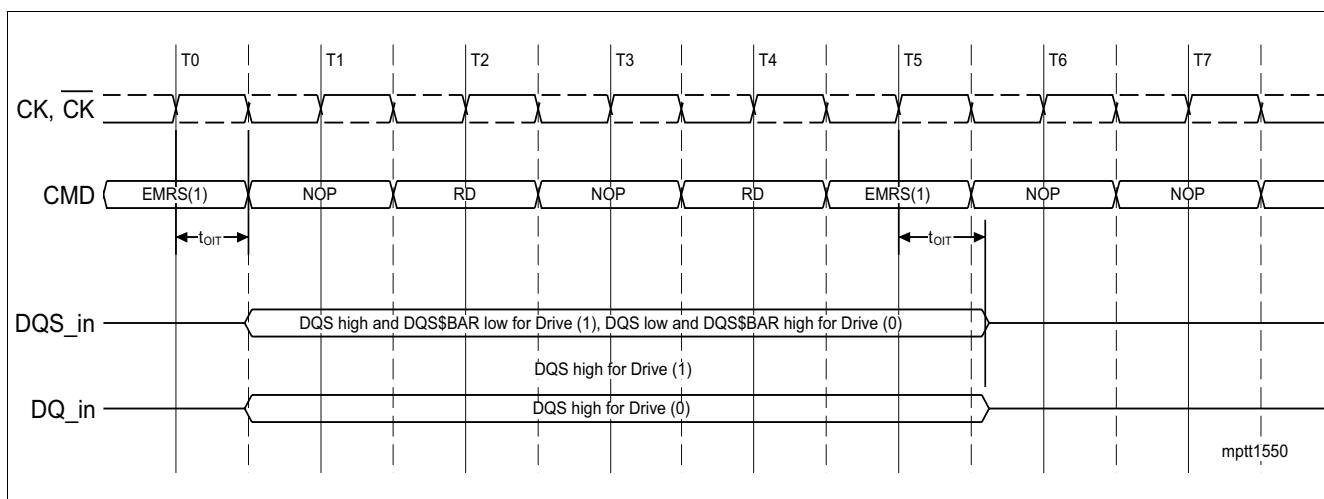
Figure 11 Timing Diagram Drive Mode
