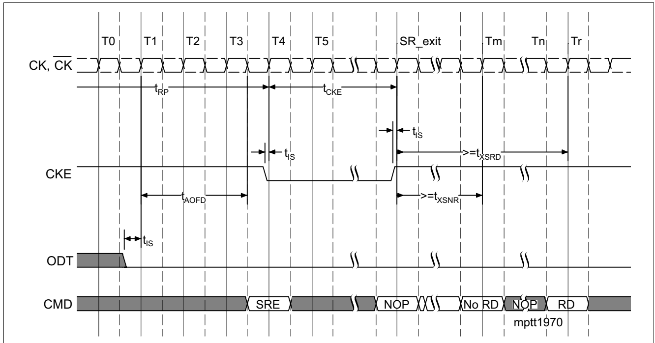
Figure 54 Self Refresh Timing
