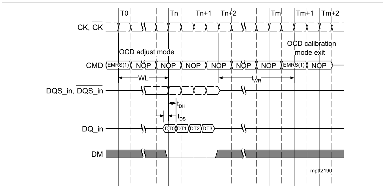
Figure 10 Timing Diagram Adjust Mode
