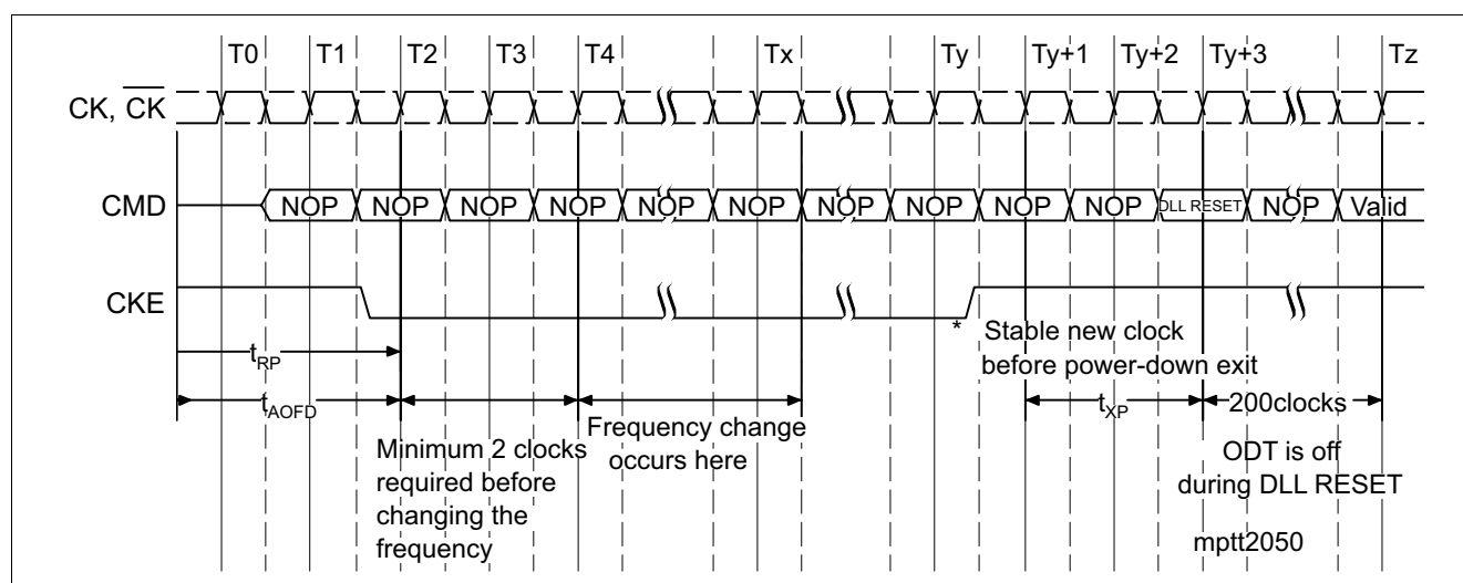
Figure 62 Input Frequency Change Example during Precharge Power-Down mode
