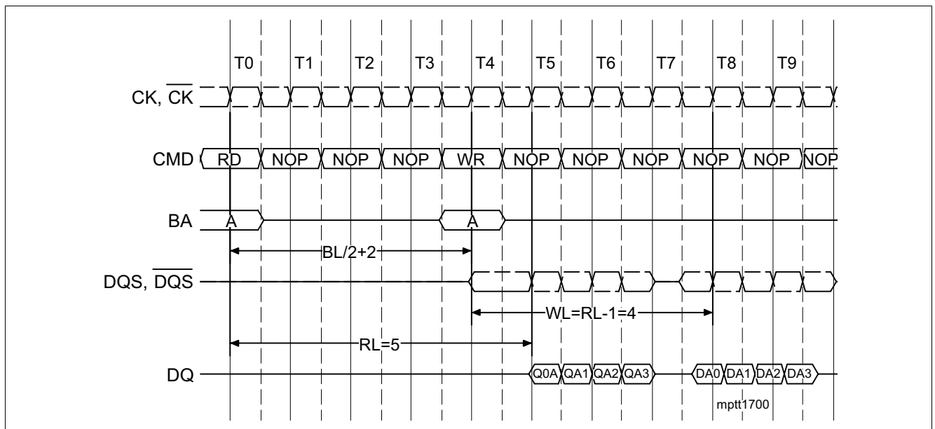
Figure 27 Read followed by Write Ex. RL = 5 , WL = (RL-1) = 4 , BL = 4
