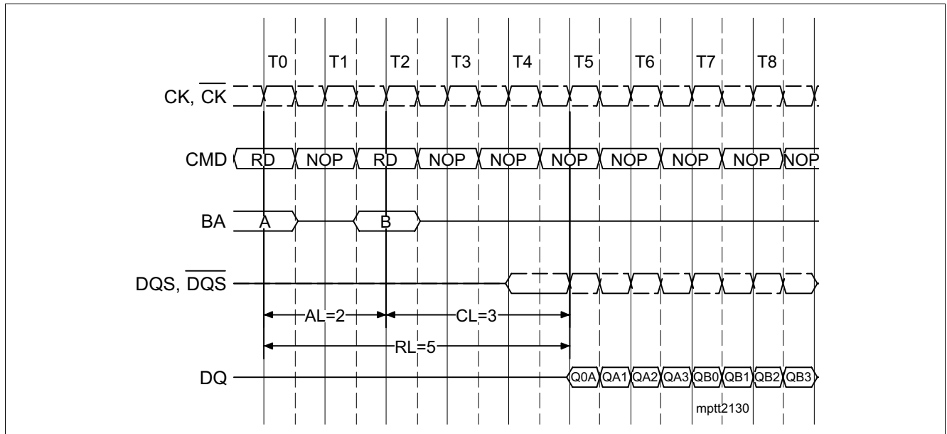
Figure 28 Seamless Read Operation Ex. 1 RL = 5 , AL = 2 , CL = 3 , BL = 4
