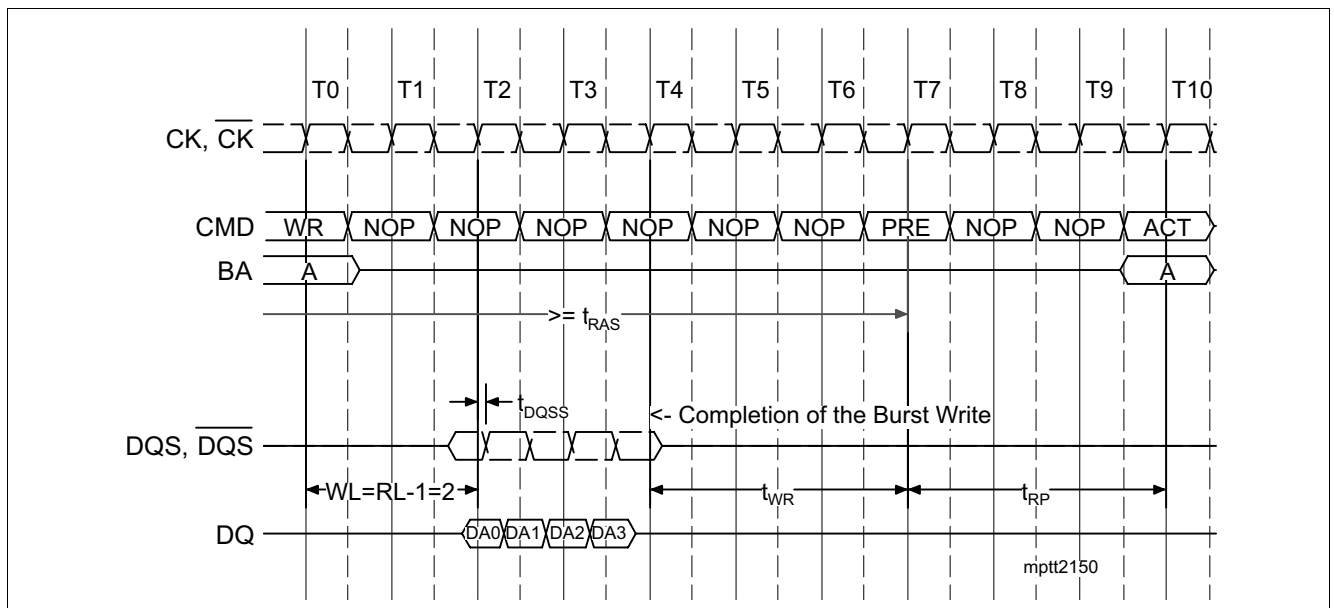
Figure 32 Write Operation Ex. 2 RL = 3 (AL = 0, CL = 3), WL = 2, BL = 4
