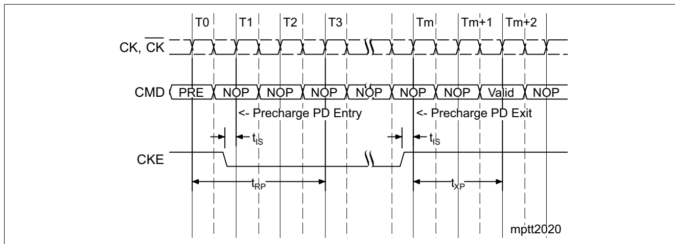
Figure 59 Precharge Power Down Mode Entry and Exit
