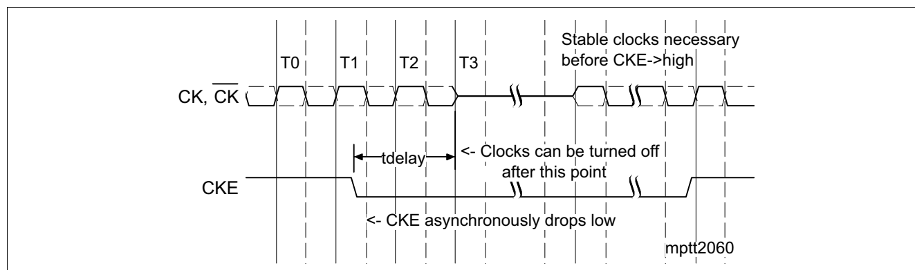
Figure 63 Asynchronous Low Reset Event
