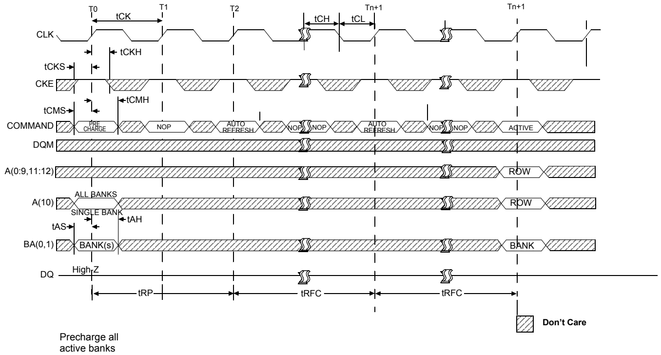
Figure 34: Auto-Refresh Mode
