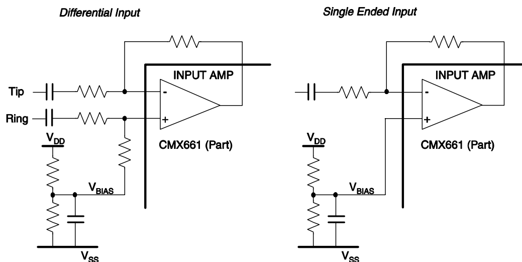
Figure 3: Example Input Configurations
