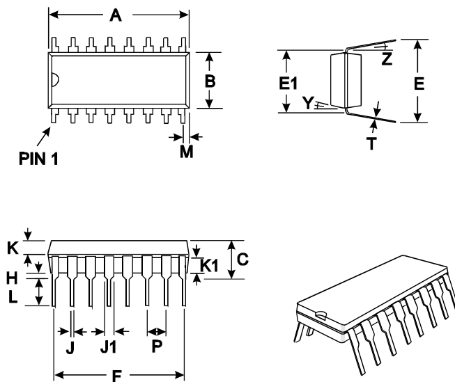
Figure 6: D4 Mechanical Outline: Order as part no. CMX661D4
