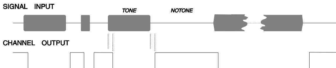
Figure 4: Detector Output Format
