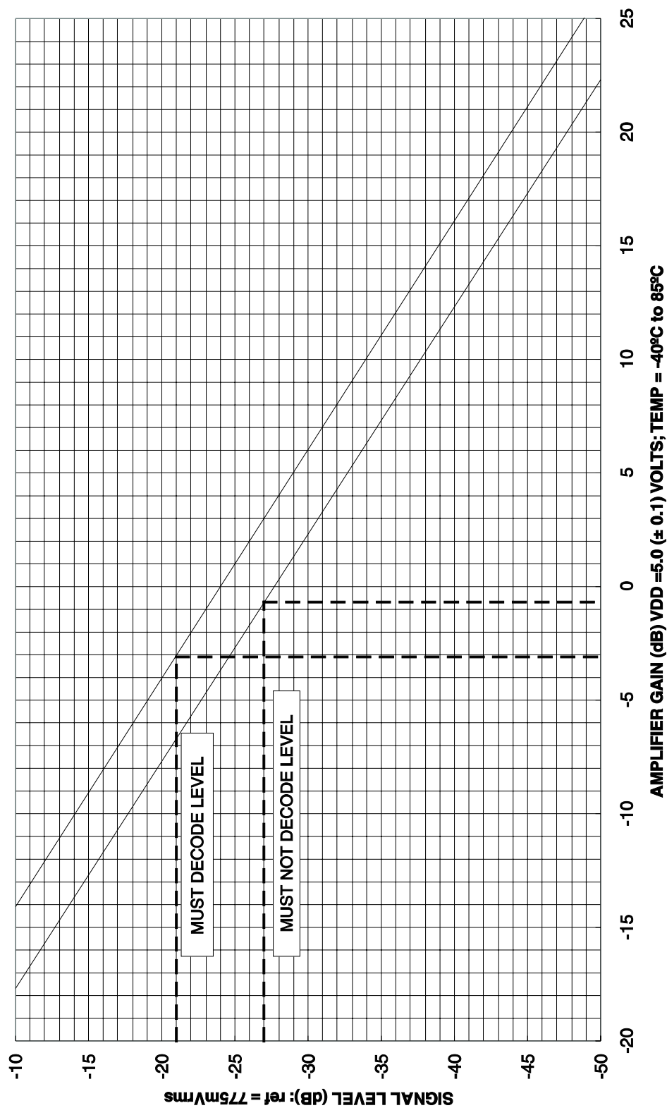
Figure 5: Input Gain Calculation Graph
