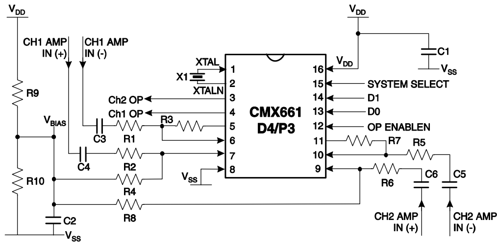
Figure 2: Typical External Components
