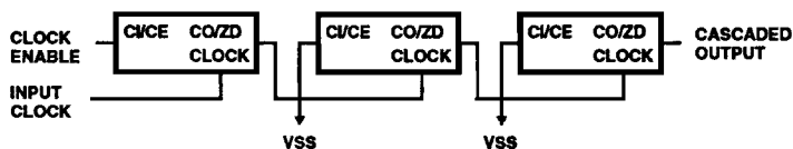
FIGURE 17. RIPPLE CASCADED
