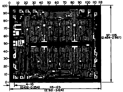
CD40103BMS
