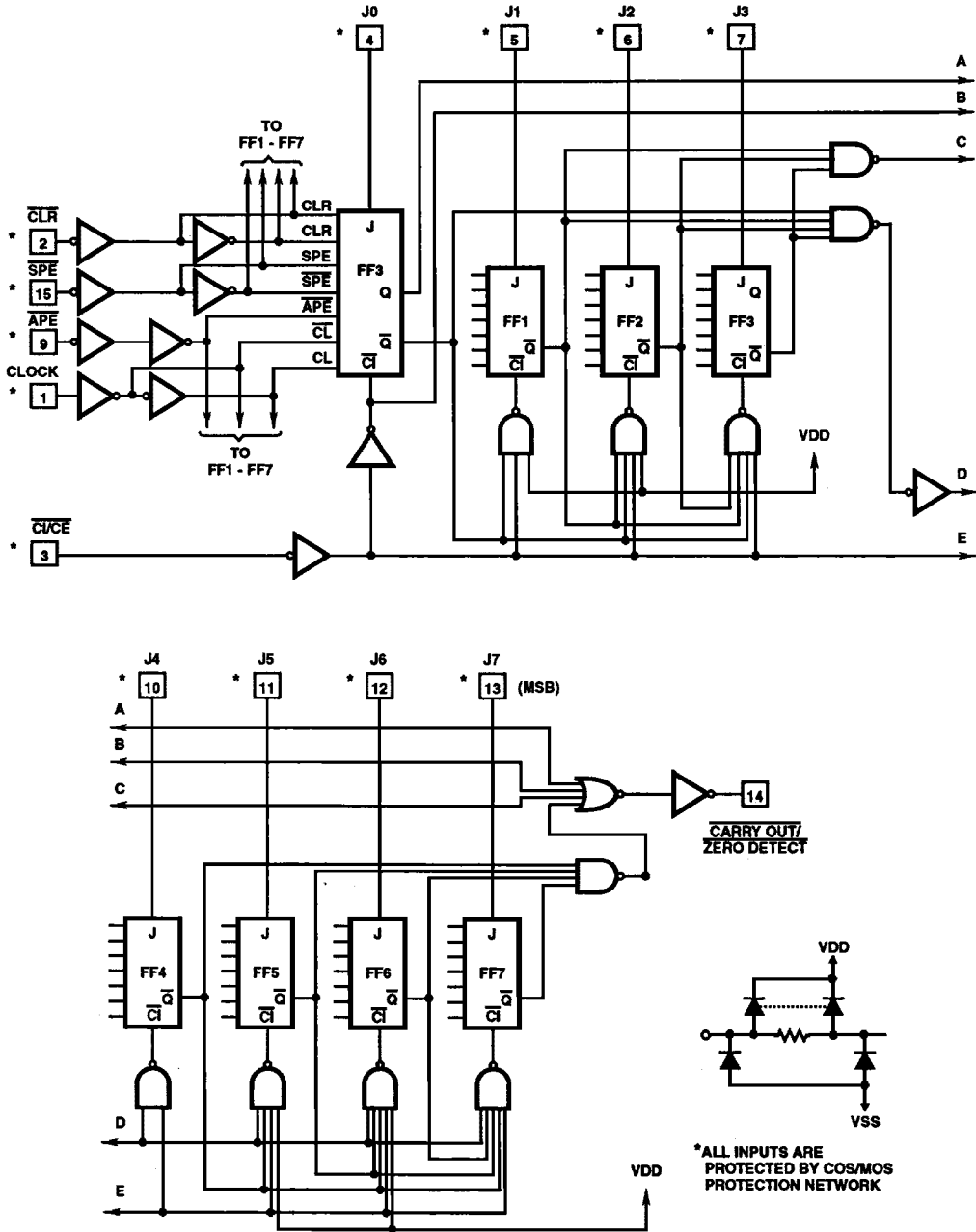
FIGURE 2. LOGIC DIAGRAM FOR CD40103BMS
