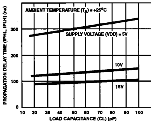
FIGURE 8. TYPICAL PROPAGATION DELAY TIME AS A FUNCTION OF LOAD CAPACITANCE (CLOCK TO C_O/ZD )
