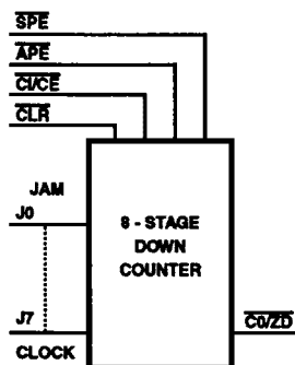
CD40102BMS, CD40103BMS
