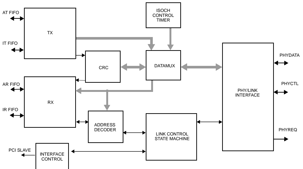
Figure 4. Link Core Block Diagram
