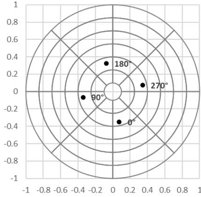
Vector Modulator Insertion Loss vs Phase: 10GHz (dB)
